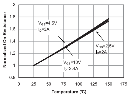
Figure 4: On-Resistance vs. Junction Temperature (Note E)
