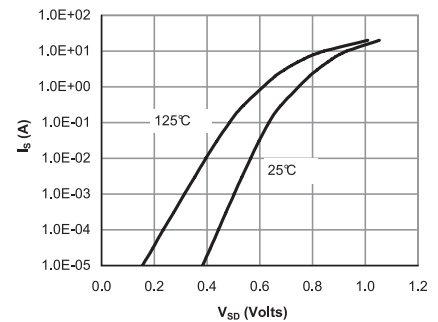
Figure 6: Body-Diode Characteristics (Note E)
