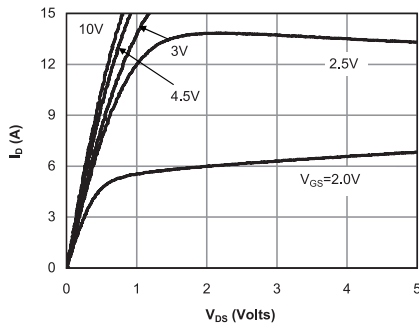
Figure 1: On-Region Characteristics (Note E)
