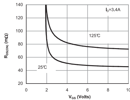
Figure 5: On-Resistance vs. Gate-Source Voltage (Note E)
