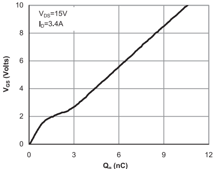
Figure 7: Gate-Charge Characteristics
