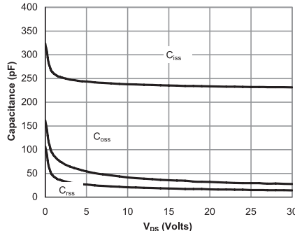
Figure 8: Capacitance Characteristics
