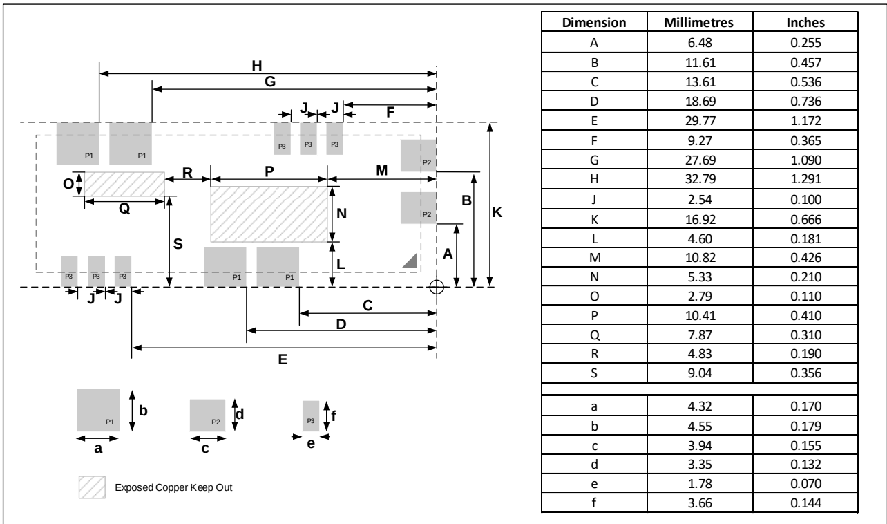
Figure 16: Land Pattern
