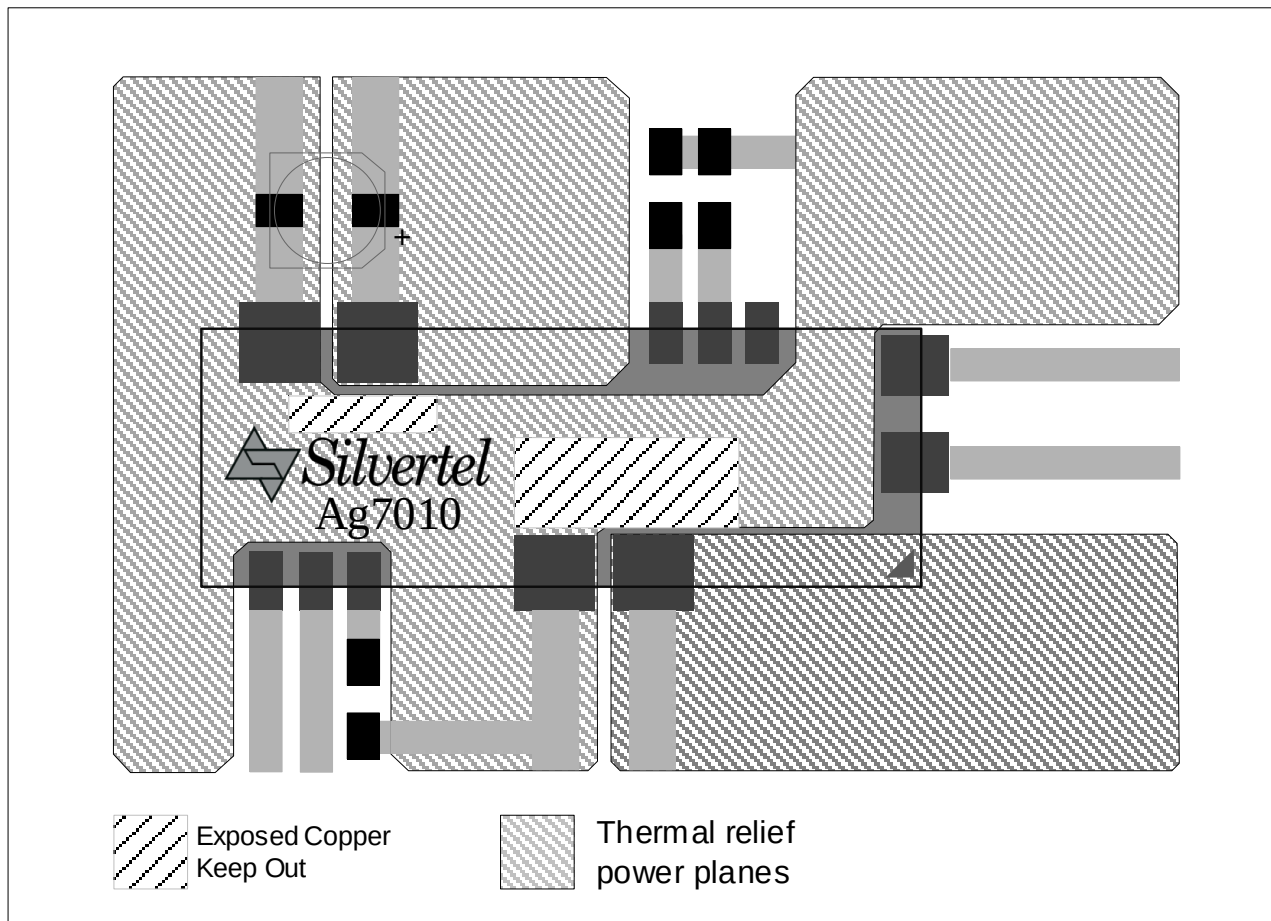
Figure 12: Thermal Relief
