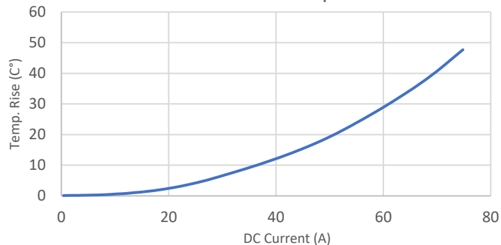
AVR-1Z100506S Series Temperature Rise
