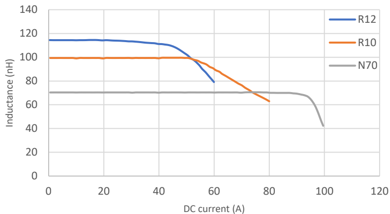
AVR-1Z100506S Series Saturation Graphs @25°C
