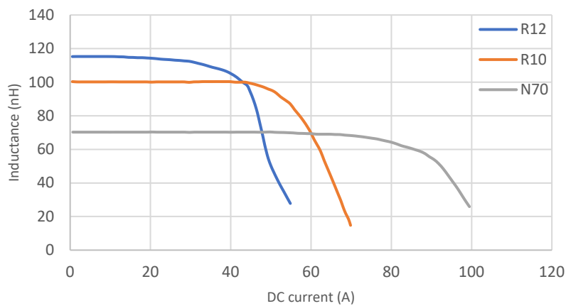
AVR-1Z100506S Series Saturation Graphs @100°C
