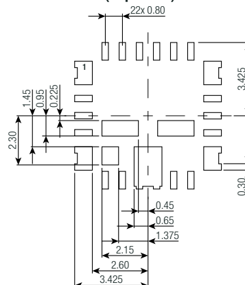
Recommended Footprint Details (Top View)
