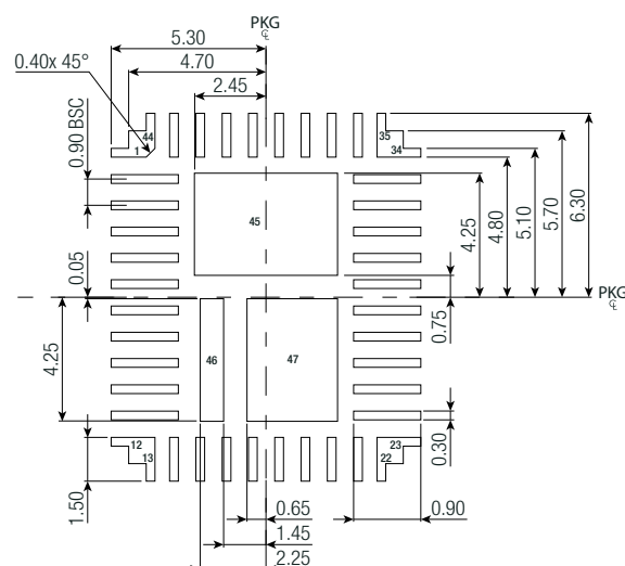
Recommended Footprint Details (Top View)
