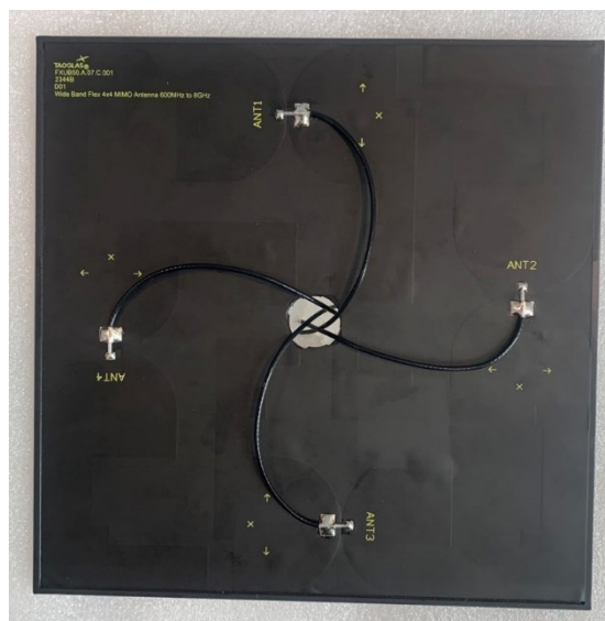
A close up to show the cable routing for the 'Inner' set-up
