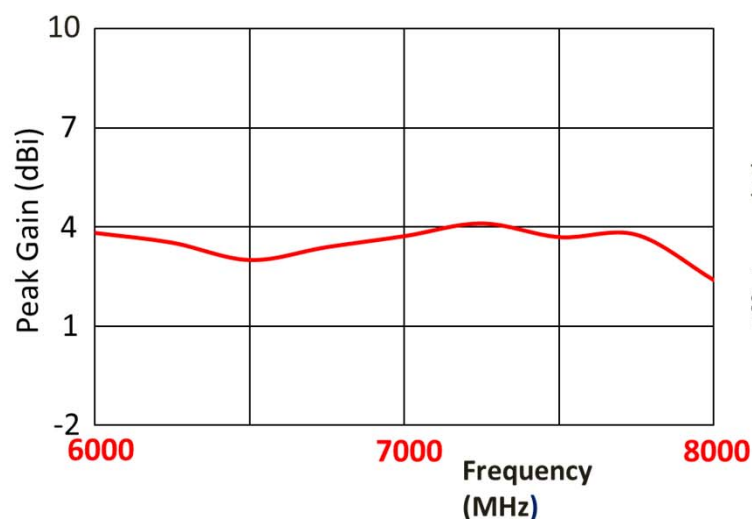
Peak Gain
