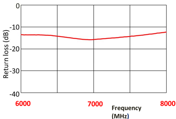
Return Loss
