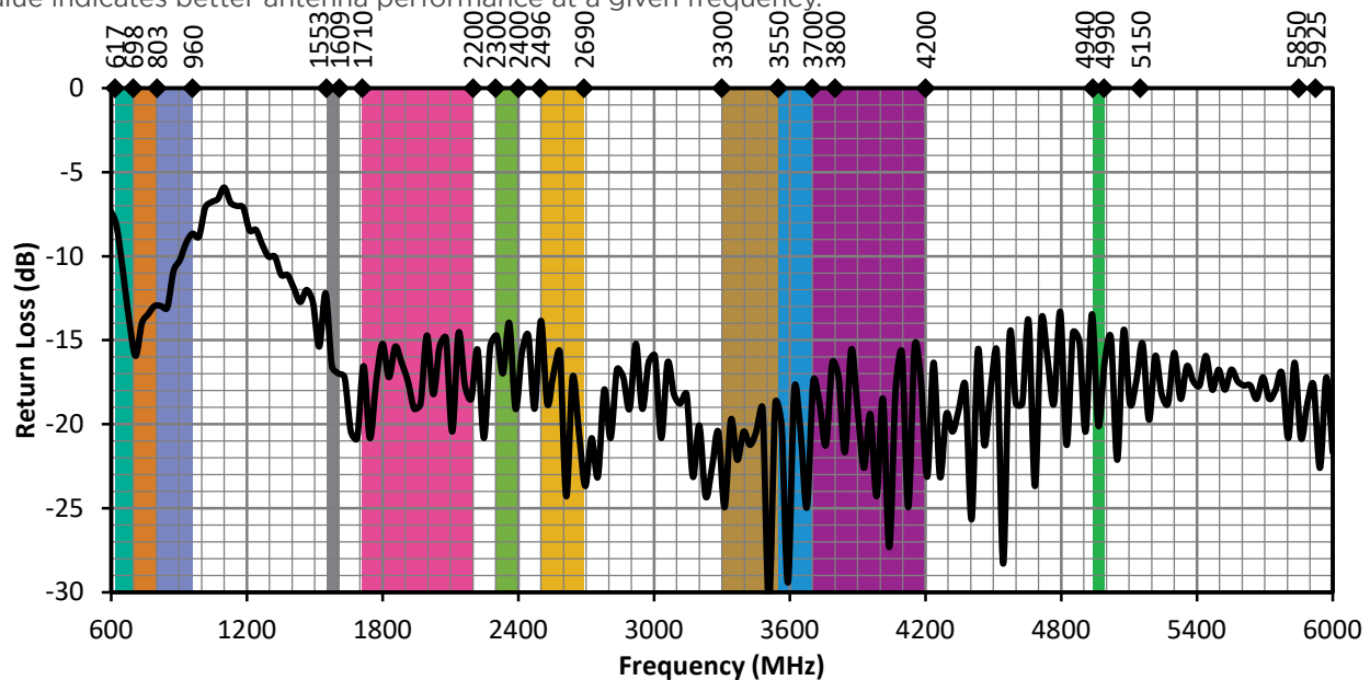
Figure 3. L9000176-01 Return Loss with Frequency Band Highlights
