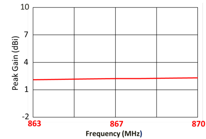
Peak Gain
