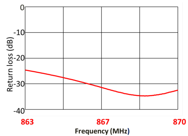
Return Loss
