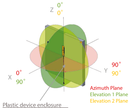
Test setup
