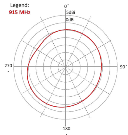
Azimuth
