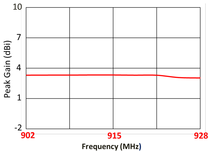
Peak Gain
