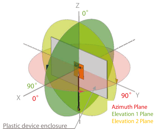
Test setup
