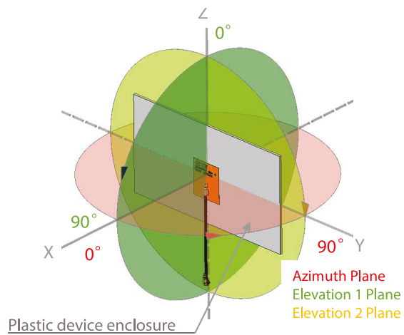
Test setup
