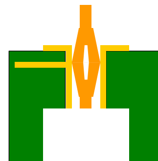
Figure 6: Counterbored Via
