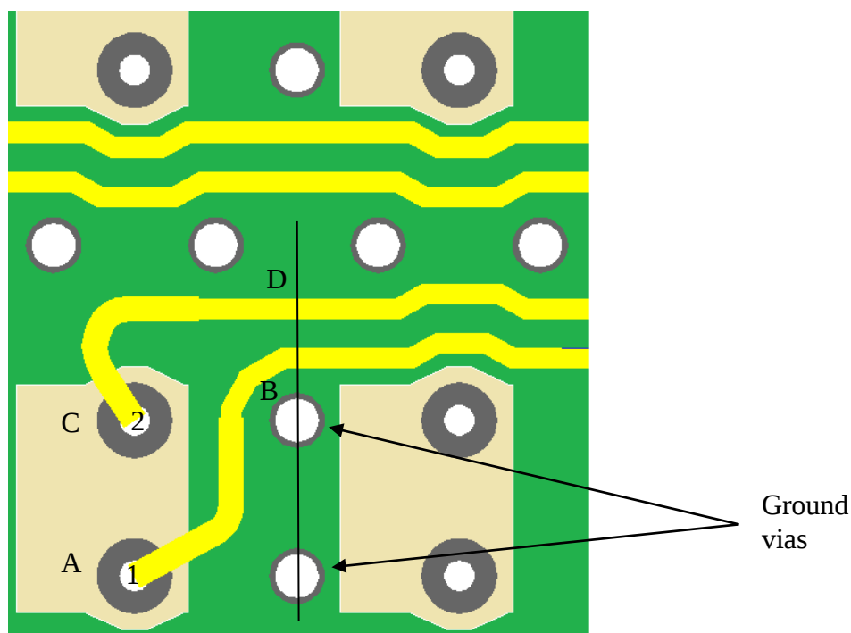
Figure 9: Example Breakout
