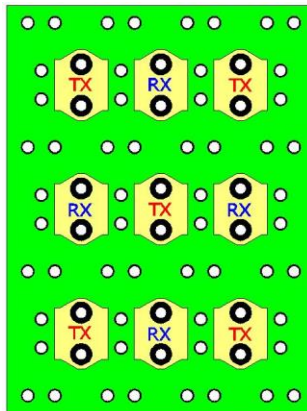
Figure 12: Interstitial Pinout
