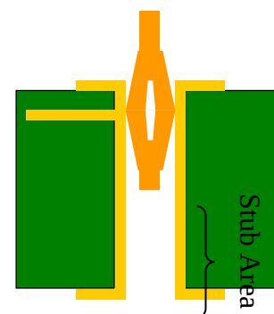
Figure 5: Via Stub
