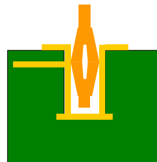
Figure 7: Blind Via
