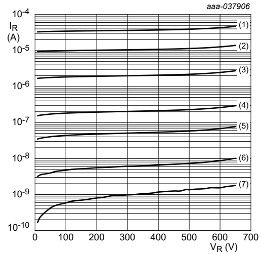
pulsed condition (1) T_j = 175\text{ °C} (2) T_j = 150\text{ °C} (3) T_j = 125\text{ °C} (4) T_j = 100\text{ °C} (5) T_j = 85\text{ °C} (6) T_j = 55\text{ °C} (7) T_j = 25\text{ °C}
