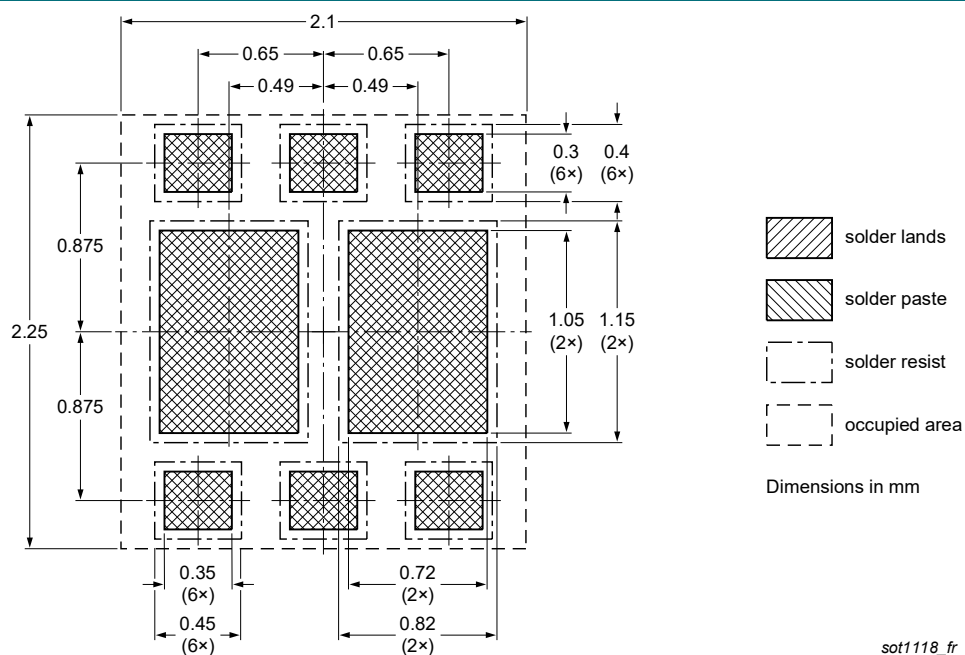
Fig. 30. Reflow soldering footprint for DFN2020-6 (SOT1118)
