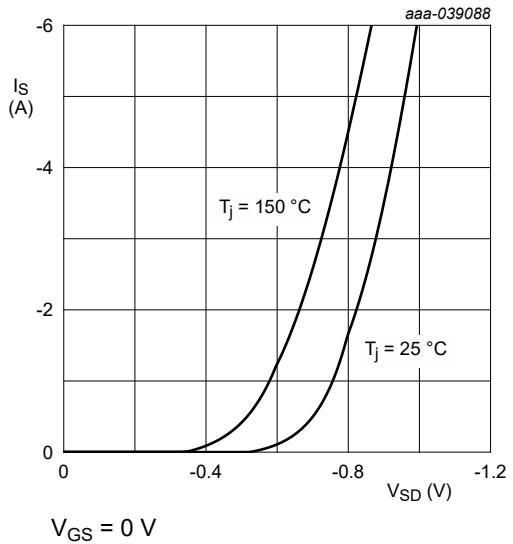
Fig. 27. TR2: Source current as a function of source-drain voltage; typical values
