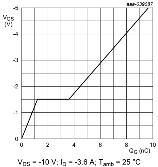
Fig. 26. TR2: Gate-source voltage as a function of gate charge; typical values
