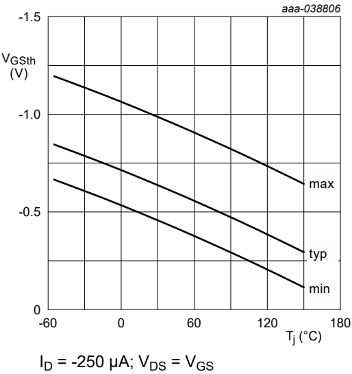
Fig. 24. TR2: Gate-source threshold voltage as a function of junction temperature
