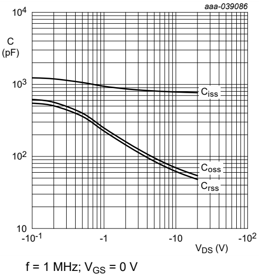
Fig. 25. TR2: Input, output and reverse transfer capacitances as a function of drain-source voltage; typical values
