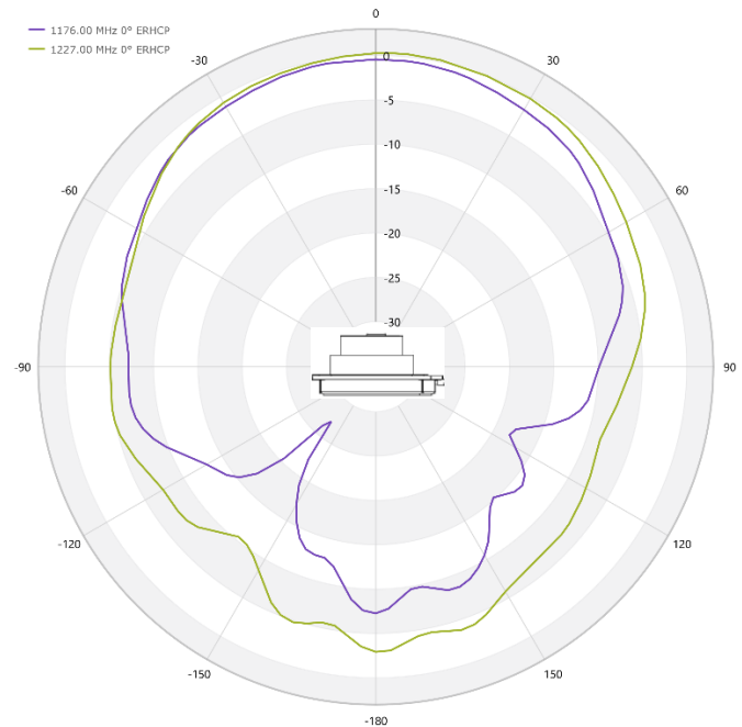
L2 + L5 RHCP Pattern
