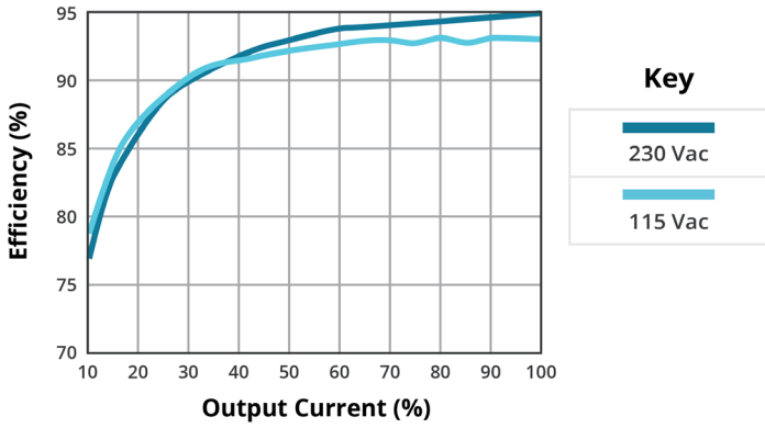
EFFICIENCY VS OUTPUT LOAD TJ-100-28
