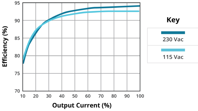
EFFICIENCY VS OUTPUT LOAD TJ-100-12
