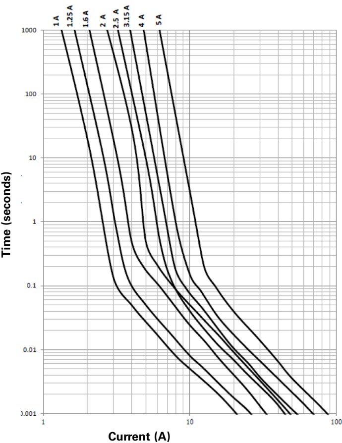
Current vs. time curve
