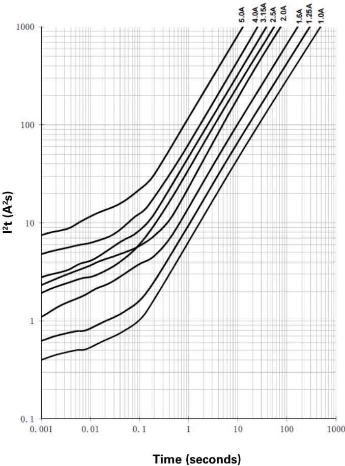
I²t vs. time curve
