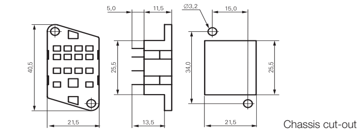
Chassis cut-out
