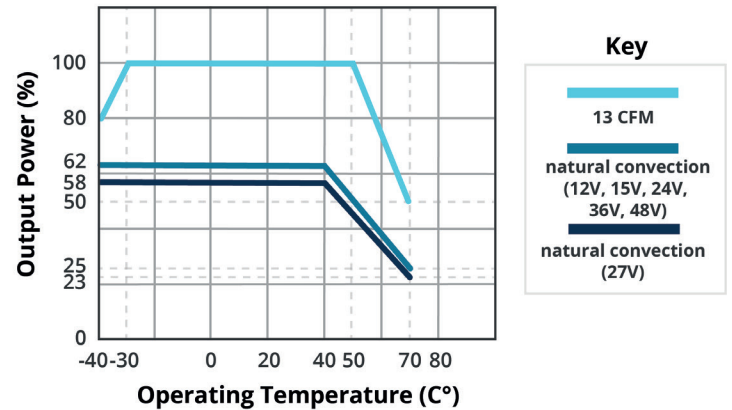
TEMPERATURE DERATING CURVE (-CNF versions)
