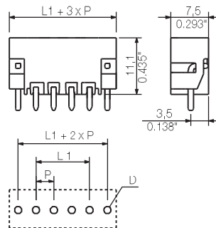
Dimensioned drawing
