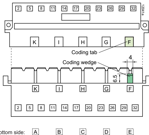
Fig. 18 Integrated code key system (H11 connector)
