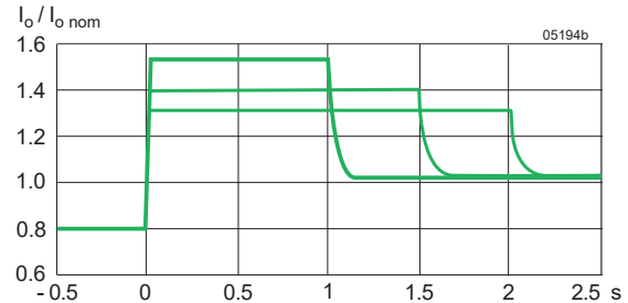
Fig. 8 Short term peak power characteristic: overcurrent versus time (typical values).
