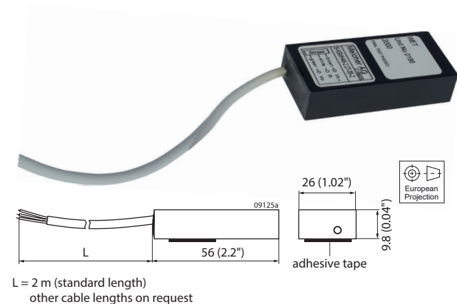
Fig. 26 Temperature sensor
