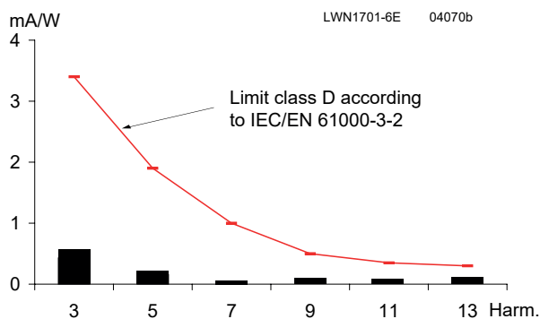
Fig. 4 Harmonic currents at input current, measured at V_i = 230 \text{ VAC} , I_o = I_{o \text{ nom}} (LWN1701-6E).
