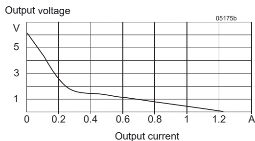
Fig. 21 Output voltage versus output current, while the shutdown is activated ( V_i = V_{i \text{ nom}} ).
