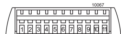
Fig. 15b View of the output terminals (cage clamp style)
