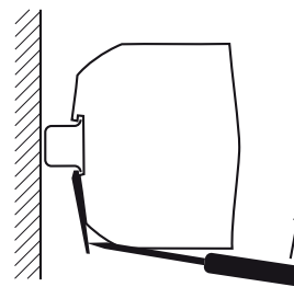
Fig. 16b Dismounting from DIN-rail. Use proper tool (min. 3 mm screwdriver) and adequate force.
