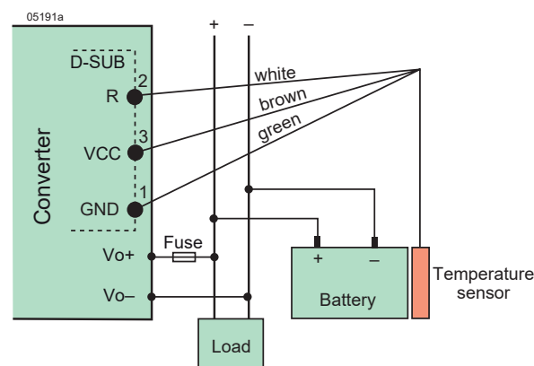
Fig. 27 Connection of temperature sensor
