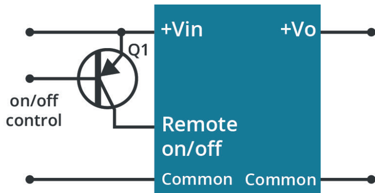
Figure 7 Negative Remote On/Off Input Drive Circuit
