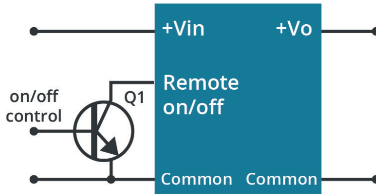
Figure 6 Positive Remote on/off Input Drive Circuit
