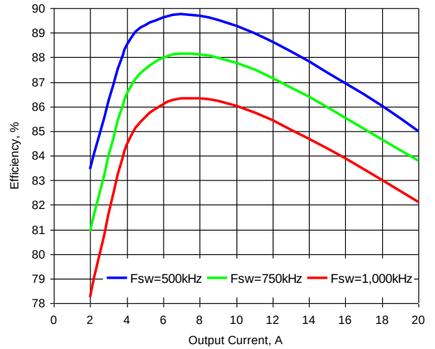
Figure 8. Efficiency vs. Load. Vin=5V, Vout=1.2V
