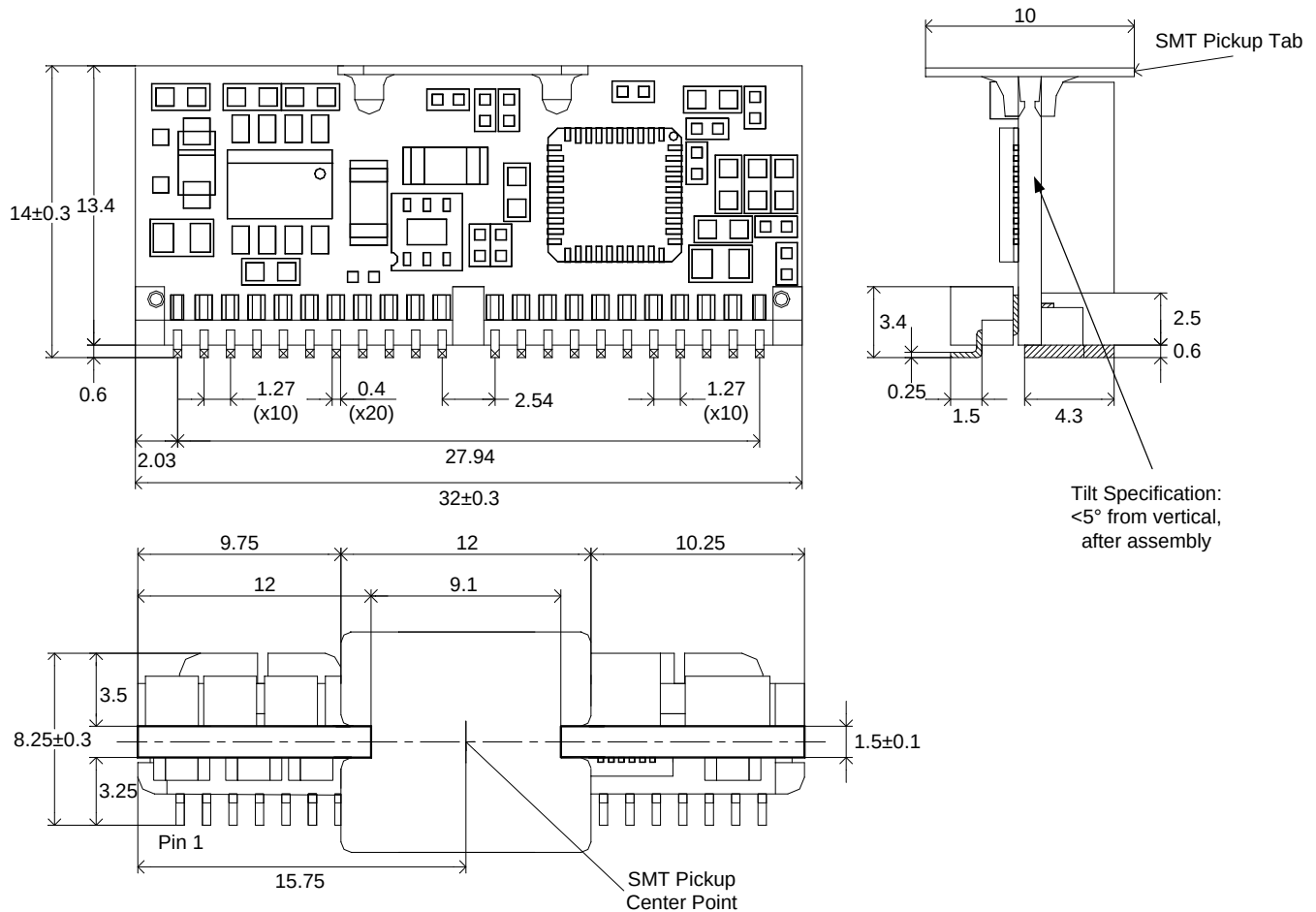
Figure 57. Mechanical Drawing
