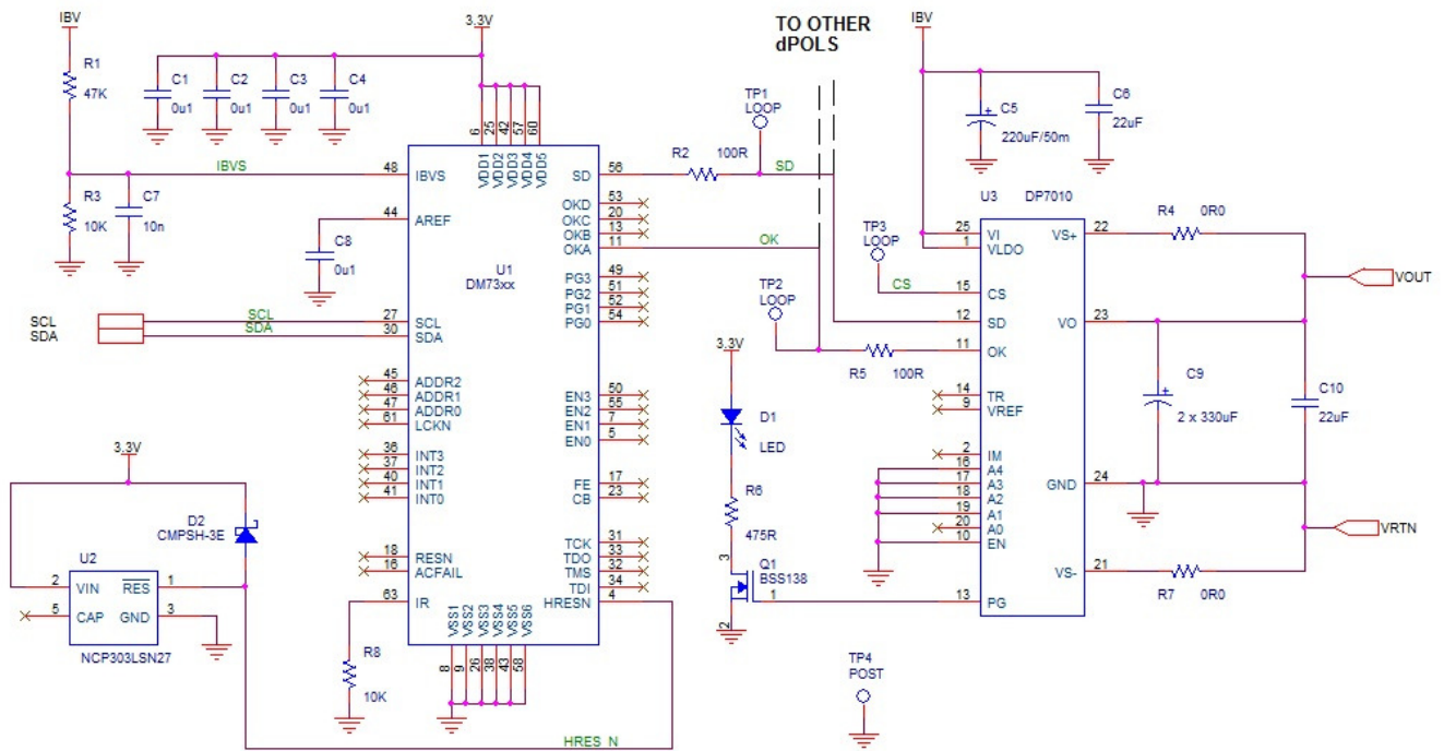
Figure 51. Typical Application with Digital Power Manager and I 2 C Interface
