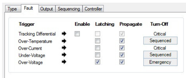
Figure 27. GUI dPOL Fault Propagation Option Window
