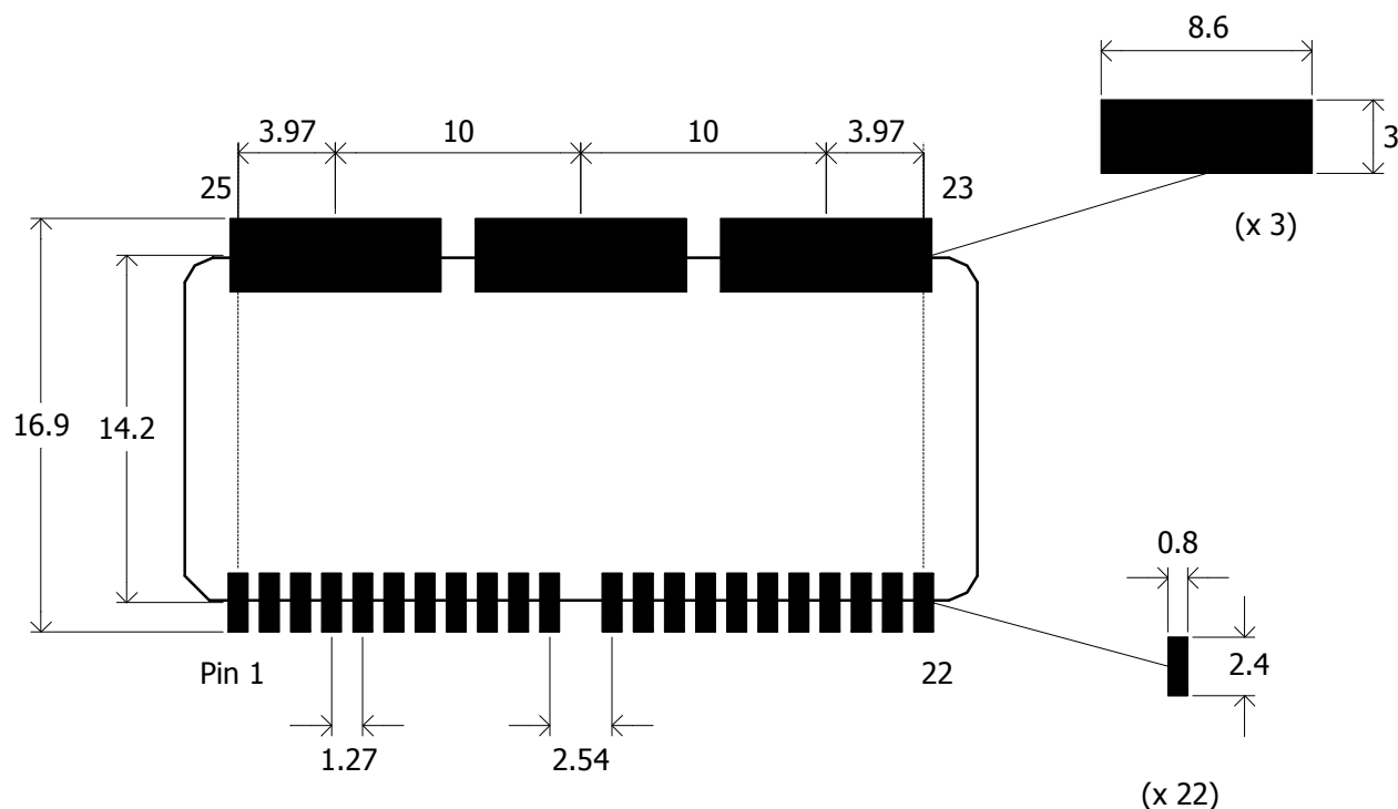
Figure 53. Recommended PCB Pad Sizes
