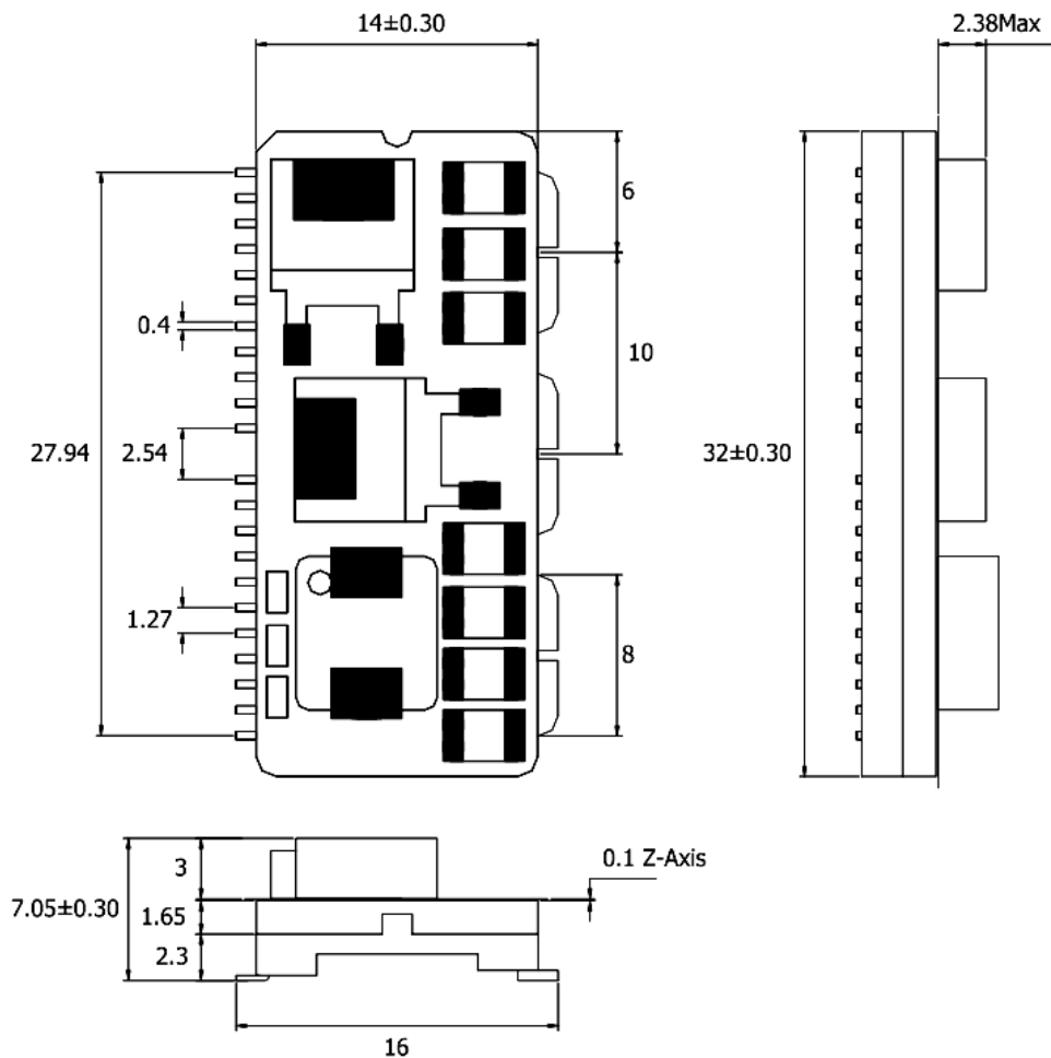
Figure 52. Top (Left) and Bottom Views
