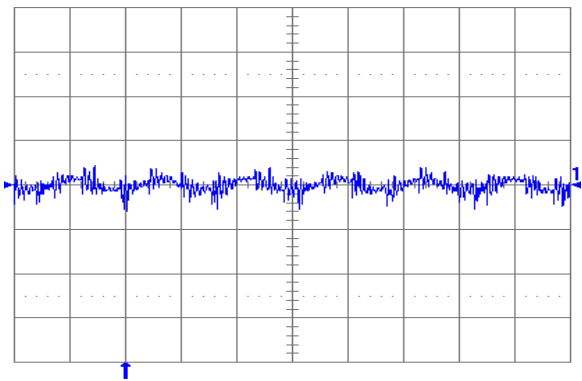
Fig. 1.5V.6: Output voltage ripple (20 mV/div.) at full rated load current into a resistive load with external capacitance 100\text{ }\mu\text{F} ceramic + 1\text{ }\mu\text{F} ceramic and V_{in} = 5\text{ V} for V_{out} = 1.5\text{ V} . Time scale: 2 \mu\text{s} /div.
