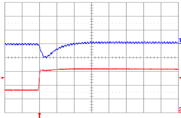
Fig. 2.5V.6: Output voltage response for V_{out} = 2.5\text{ V} to positive load current step change from 8 A to 16 A with slew rate of 5\text{ A}/\mu\text{s} at V_{in} = 12\text{ V} . Top trace: output voltage (200 mV/div.); Bottom trace: load current (5 A/div.). C_o = 100\text{ }\mu\text{F} ceramic. Time scale: 20 μs/div.
