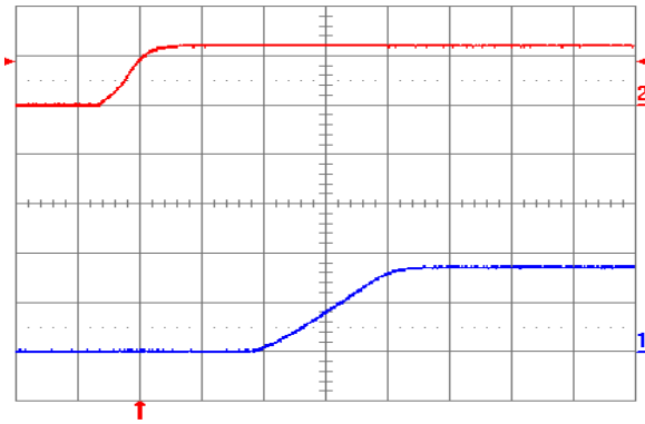
Fig. 1.8V.4: Turn-on transient for V_{out} = 1.8\text{ V} with application of V_{in} at full rated load current (resistive) and 100\text{ }\mu\text{F} external capacitance at V_{in} = 12\text{ V} . Top trace: V_{in} ( 10\text{ V/div.} ); Bottom trace: output voltage ( 1\text{ V/div.} ); Time scale: 2\text{ ms/div.}
