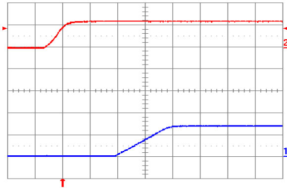
Fig. 0.7525V.4: Turn-on transient for V_{out} = 0.7525 V with application of V_{in} at full rated load current (resistive) and 100\ \mu\text{F} external capacitance at V_{in} = 12 V. Top trace: V_{in} (10 V/div.); Bottom trace: output voltage (0.5 V/div.); Time scale: 2 ms/div.
