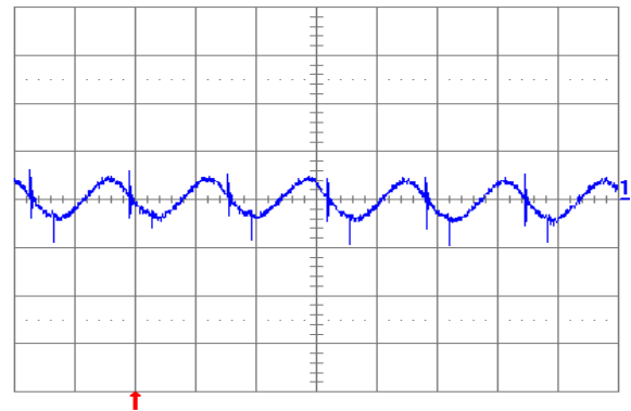
Fig. 2.5V.5: Output voltage ripple (20 mV/div.) at full rated load current into a resistive load with external capacitance 100\text{ }\mu\text{F} ceramic and V_{in} = 12\text{ V} for V_{out} = 2.5\text{ V} . Time scale: 2 μs/div.
