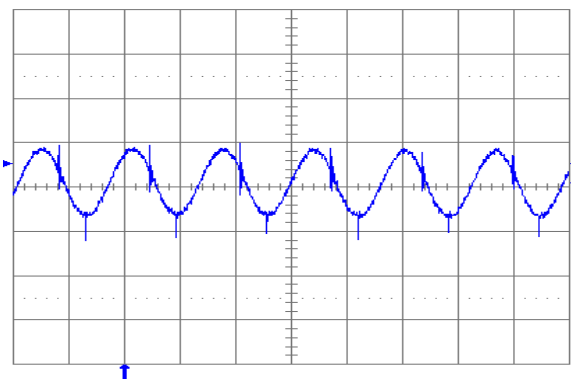
Fig. 3.3V.5: Output voltage ripple ( 20\text{ mV/div.} ) at full rated load current into a resistive load with external capacitance 100\text{ }\mu\text{F} ceramic and V_{in} = 12\text{ V} for V_{out} = 3.3\text{ V} . Time scale: 2\text{ }\mu\text{s/div.}
