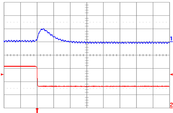
Fig. 2.5V.7: Output voltage response for V_{out} = 2.5\text{ V} to negative load current step change from 16 A to 8 A with slew rate of -5\text{ A}/\mu\text{s} at V_{in} = 12\text{ V} . Top trace: output voltage (200 mV/div.); Bottom trace: load current (5 A/div.). C_o = 100\text{ }\mu\text{F} ceramic. Time scale: 20 μs/div.
