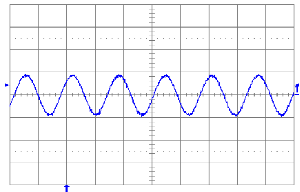
Fig. 5.0V.5: Output voltage ripple (20 mV/div.) at full rated load current into a resistive load with external capacitance 100 \mu\text{F} ceramic and V_{in} = 12 V for V_{out} = 5.0 V. Time scale: 2 μs/div.
