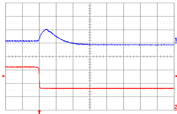
Fig. 0.7525V.7: Output voltage response for V_{out} = 0.7525 V to negative load current step change from 16 A to 8 A with slew rate of -5\ \text{A}/\mu\text{s} at V_{in} = 12 V. Top trace: output voltage (200 mV/div.); Bottom trace: load current (5 A/div.). C_o = 100\ \mu\text{F} ceramic. Time scale: 20 \mu\text{s} /div.
