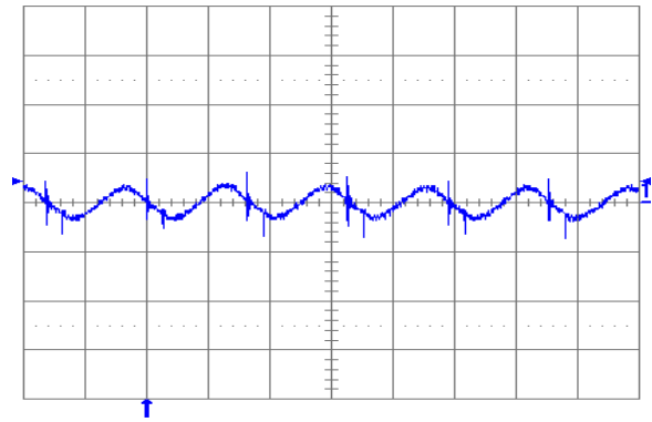
Fig. 1.8V.5: Output voltage ripple ( 20\text{ mV/div.} ) at full rated load current into a resistive load with external capacitance 100\text{ }\mu\text{F} ceramic and V_{in} = 12\text{ V} for V_{out} = 1.8\text{ V} . Time scale: 2\text{ }\mu\text{s/div.}
