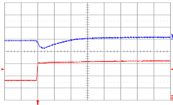
Fig. 0.7525V.6: Output voltage response for V_{out} = 0.7525 V to positive load current step change from 8 A to 16 A with slew rate of 5\ \text{A}/\mu\text{s} at V_{in} = 12 V. Top trace: output voltage (200 mV/div.); Bottom trace: load current (5 A/div.). C_o = 100\ \mu\text{F} ceramic. Time scale: 20 \mu\text{s} /div.
