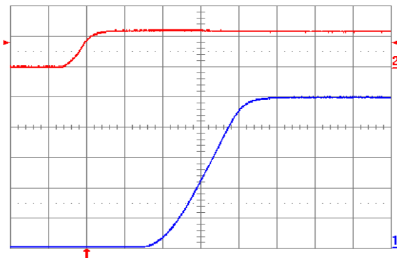
Fig. 5.0V.4: Turn-on transient for V_{out} = 5.0 V with application of V_{in} at full rated load current (resistive) and 100 \mu\text{F} external capacitance at V_{in} = 12 V. Top trace: V_{in} (10 V/div.); Bottom trace: output voltage (1 V/div.); Time scale: 2 ms/div.
