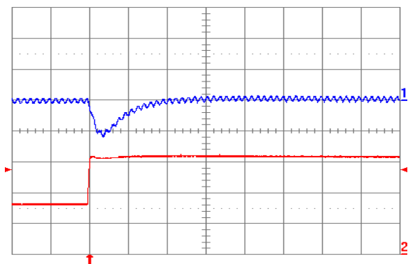
Fig. 3.3V.6: Output voltage response for V_{out} = 3.3\text{ V} to positive load current step change from 8\text{ A} to 16\text{ A} with slew rate of 5\text{ A}/\mu\text{s} at V_{in} = 12\text{ V} . Top trace: output voltage ( 200\text{ mV/div.} ); Bottom trace: load current ( 5\text{ A/div.} ). C_o = 100\text{ }\mu\text{F} ceramic. Time scale: 20\text{ }\mu\text{s/div.}
