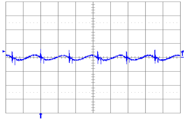
Fig. 1.0V.5: Output voltage ripple ( 20\text{ mV/div.} ) at full rated load current into a resistive load with external capacitance 100\text{ }\mu\text{F} ceramic and V_{in} = 12\text{ V} for V_{out} = 1.0\text{ V} . Time scale: 2\text{ }\mu\text{s/div.}
