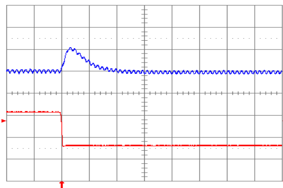
Fig. 3.3V.7: Output voltage response for V_{out} = 3.3\text{ V} to negative load current step change from 16\text{ A} to 8\text{ A} with slew rate of -5\text{ A}/\mu\text{s} at V_{in} = 12\text{ V} . Top trace: output voltage ( 200\text{ mV/div.} ); Bottom trace: load current ( 5\text{ A/div.} ). C_o = 100\text{ }\mu\text{F} ceramic. Time scale: 20\text{ }\mu\text{s/div.}
