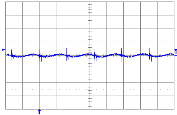
Fig. 0.7525V.5: Output voltage ripple (20 mV/div.) at full rated load current into a resistive load with external capacitance 100\ \mu\text{F} ceramic and V_{in} = 12 V for V_{out} = 0.7525 V. Time scale: 2 \mu\text{s} /div.
