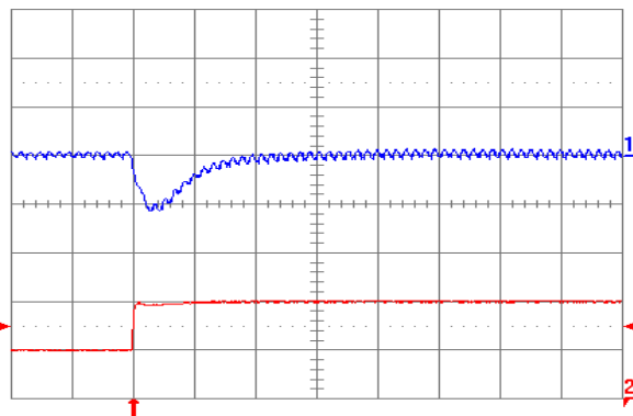
Fig. 2.0V.7: Output voltage response for V_{out} = 2.0 V to positive load current step change from 5 A to 10 A with slew rate of 5 A/ \mu s at V_{in} = 5 V. Top trace: output voltage (100 mV/div.); Bottom trace: load current (5 A/div.). C_o = 47 \mu F ceramic + 1 \mu F ceramic. Time scale: 20 \mu s/div.
