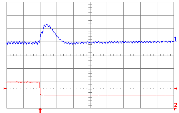
Fig. 1.2V.8: Output voltage response for V_{out} = 1.2 V to negative load current step change from 10 A to 5 A with slew rate of -5 A/ \mu s at V_{in} = 5 V. Top trace: output voltage (100 mV/div.); Bottom trace: load current (5 A/div.). C_o = 47 \mu F ceramic + 1 \mu F ceramic. Time scale: 20 \mu s/div.
