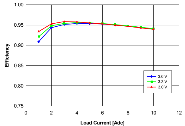
Fig. 2.5V.4: Efficiency vs. load current and input voltage for V_{out} = 2.5 V converter mounted vertically with air flowing at a rate of 200 LFM (1 m/s) and T_a = 25 °C.
