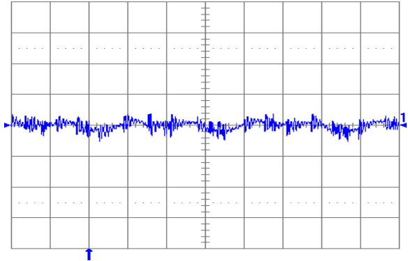
Fig. 0.7525V.6: Output voltage ripple (20 mV/div.) at full rated load current into a resistive load with external capacitance 47 \mu\text{F} ceramic + 1 \mu\text{F} ceramic, and V_{in} = 5 V for V_{out} = 0.7525 V. Time scale: 2 \mu\text{s} /div.
