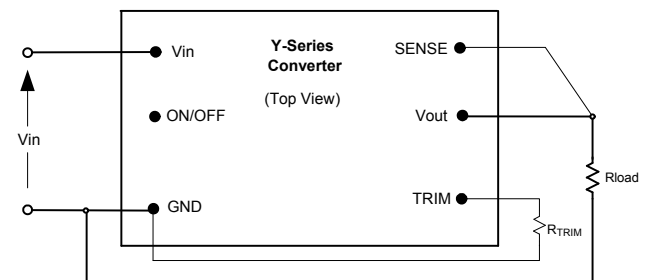
Fig. E: Configuration for programming output voltage.
