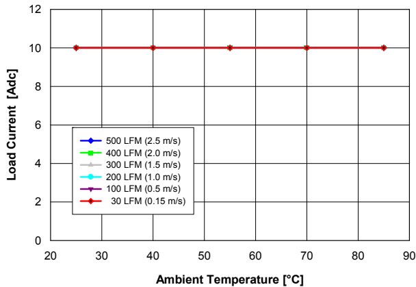
Fig. 1.8V.1: Available load current vs. ambient temperature and airflow rates for V_{out} = 1.8 V converter mounted vertically with V_{in} = 5 V, and maximum MOSFET temperature \leq 120 °C.
