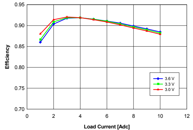
Fig. 1.2V.4: Efficiency vs. load current and input voltage for Vout = 1.2 V converter mounted vertically with air flowing at a rate of 200 LFM (1 m/s) and Ta = 25 °C.
