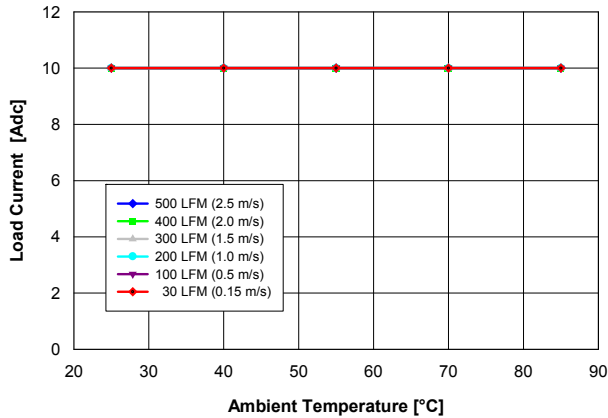
Fig. 2.0V.1: Available load current vs. ambient temperature and airflow rates for Vout = 2.0 V converter mounted vertically with Vin = 5 V, and maximum MOSFET temperature ≤ 120 °C.
