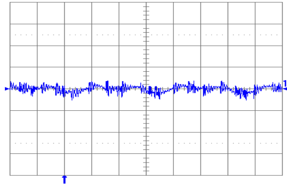
Fig. 1.0V.6: Output voltage ripple (20 mV/div.) at full rated load current into a resistive load with external capacitance 47 \mu\text{F} ceramic + 1 \mu\text{F} ceramic, and V_{in} = 5 V for V_{out} = 1.0 V. Time scale: 2 \mu\text{s} /div.
