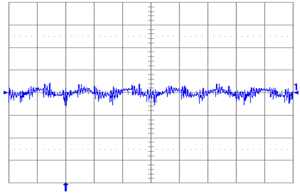
Fig. 1.5V.6: Output voltage ripple ( 20\text{ mV/div.} ) at full rated load current into a resistive load with external capacitance 47\text{ }\mu\text{F} ceramic + 1\text{ }\mu\text{F} ceramic, and V_{in} = 5\text{ V} for V_{out} = 1.5\text{ V} . Time scale: 2\text{ }\mu\text{s/div.}
