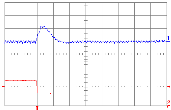
Fig. 1.5V.8: Output voltage response for V_{out} = 1.5\text{ V} to negative load current step change from 10\text{ A} to 5\text{ A} with slew rate of -5\text{ A}/\mu\text{s} at V_{in} = 5\text{ V} . Top trace: output voltage ( 100\text{ mV/div.} ); Bottom trace: load current ( 5\text{ A/div.} ). C_o = 47\text{ }\mu\text{F} ceramic + 1\text{ }\mu\text{F} ceramic. Time scale: 20\text{ }\mu\text{s/div.}
