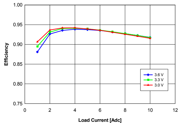
Fig. 1.8V.4: Efficiency vs. load current and input voltage for V_{out} = 1.8 V converter mounted vertically with air flowing at a rate of 200 LFM (1 m/s) and T_a = 25 °C.
