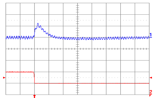
Fig. 3.3V.8: Output voltage response for V_{out} = 3.3 V to negative load current step change from 10 A to 5 A with slew rate of -5 \text{ A}/\mu\text{s} at V_{in} = 5 V. Top trace: output voltage (100 mV/div.); Bottom trace: load current (5 A/div.). C_o = 47 \mu\text{F} ceramic + 1 \mu\text{F} ceramic. Time scale: 20 \mu\text{s} /div.
