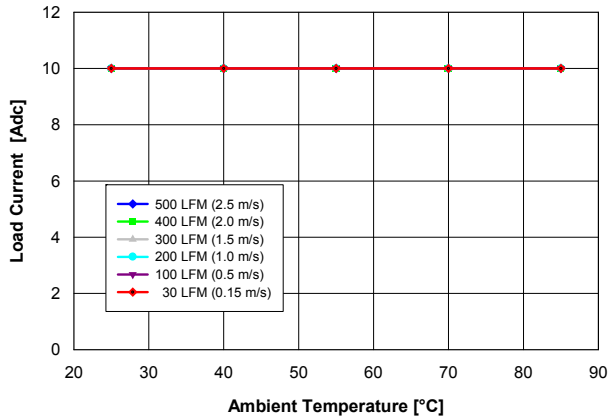
Fig. 3.3V.1: Available load current vs. ambient temperature and airflow rates for Vout = 3.3 V converter mounted vertically with Vin = 5 V, and maximum MOSFET temperature ≤ 120 °C.
