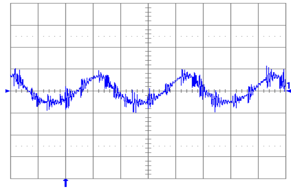
Fig. 3.3V.6: Output voltage ripple (20 mV/div.) at full rated load current into a resistive load with external capacitance 47 \mu\text{F} ceramic + 1 \mu\text{F} ceramic, and V_{in} = 5 V for V_{out} = 3.3 V. Time scale: 2 \mu\text{s} /div.
