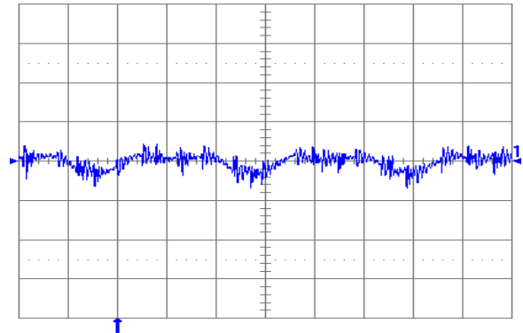
Fig. 1.2V.6: Output voltage ripple (20 mV/div.) at full rated load current into a resistive load with external capacitance 47 \mu F ceramic + 1 \mu F ceramic, and V_{in} = 5 V for V_{out} = 1.2 V. Time scale: 2 \mu s/div.
