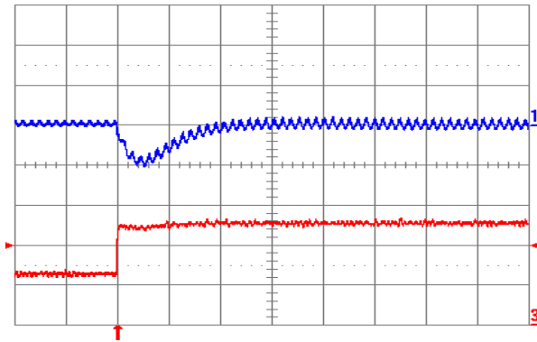
Fig. 1.0V.7: Output voltage response V_{out} = 1.0 V to positive load current step change from 5 A to 10 A with slew rate of 5 \text{ A}/\mu\text{s} at V_{in} = 5 V. Top trace: output voltage (100 mV/div.); Bottom trace: load current (5 A/div.). C_o = 47 \mu\text{F} ceramic + 1 \mu\text{F} ceramic. Time scale: 20 \mu\text{s} /div.
