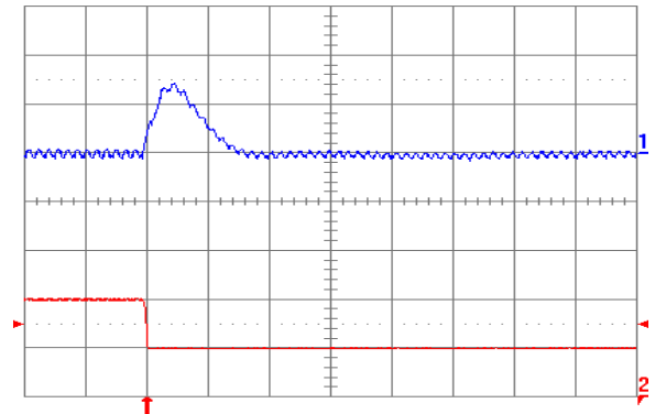
Fig. 2.0V.8: Output voltage response for V_{out} = 2.0 V to negative load current step change from 10 A to 5 A with slew rate of -5 A/ \mu s at V_{in} = 5 V. Top trace: output voltage (100 mV/div.); Bottom trace: load current (5 A/div.). C_o = 47 \mu F ceramic + 1 \mu F ceramic. Time scale: 20 \mu s/div.
