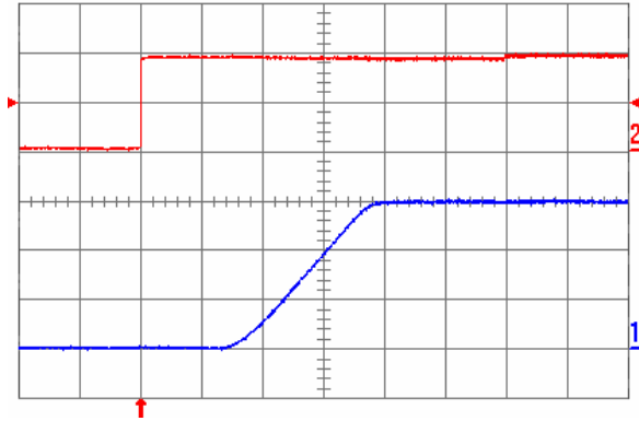
Fig. 1.5V.5: Turn-on transient for V_{out} = 1.5\text{ V} with the application of Enable signal at full rated load current (resistive) and 47\text{ }\mu\text{F} external capacitance at V_{in} = 5\text{ V} . Top trace: Enable signal ( 2\text{ V/div.} ); Bottom trace: output voltage ( 500\text{ mV/div.} ); Time scale: 2\text{ ms/div.}
