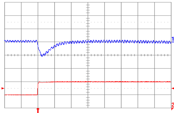
Fig. 2.5V.7: Output voltage response for V_{out} = 2.5 V to positive load current step change from 5 A to 10 A with slew rate of 5 A/ \mu s at V_{in} = 5 V. Top trace: output voltage (100 mV/div.); Bottom trace: load current (5 A/div.). C_o = 47 \mu F ceramic + 1 \mu F ceramic. Time scale: 20 \mu s/div.
