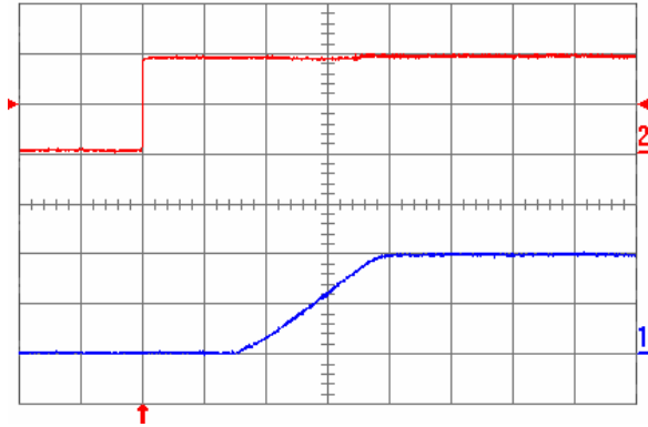
Fig. 1.0V.5: Turn-on transient for V_{out} = 1.0 V with the application of Enable signal at full rated load current (resistive) and 47 \mu\text{F} external capacitance at V_{in} = 5 V. Top trace: Enable signal (2 V/div.); Bottom trace: output voltage (500 mV/div.); Time scale: 2 ms/div.
