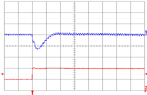
Fig. 1.5V.7: Output voltage response for V_{out} = 1.5\text{ V} to positive load current step change from 5\text{ A} to 10\text{ A} with slew rate of 5\text{ A}/\mu\text{s} at V_{in} = 5\text{ V} . Top trace: output voltage ( 100\text{ mV/div.} ); Bottom trace: load current ( 5\text{ A/div.} ). C_o = 47\text{ }\mu\text{F} ceramic + 1\text{ }\mu\text{F} ceramic. Time scale: 20\text{ }\mu\text{s/div.}
