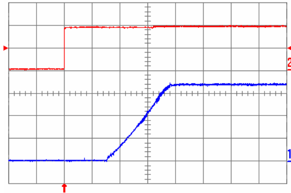
Fig. 0.7525V.5: Turn-on transient for V_{out} = 0.7525 V with the application of Enable signal at full rated load current (resistive) and 47 \mu\text{F} external capacitance at V_{in} = 5 V. Top trace: Enable signal (2 V/div.); Bottom trace: output voltage (200 mV/div.); Time scale: 2 ms/div.
