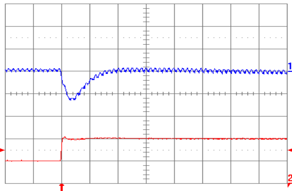
Fig. 1.2V.7: Output voltage response for V_{out} = 1.2 V to positive load current step change from 5 A to 10 A with slew rate of 5 A/ \mu s at V_{in} = 5 V. Top trace: output voltage (100 mV/div.); Bottom trace: load current (5 A/div.). C_o = 47 \mu F ceramic + 1 \mu F ceramic. Time scale: 20 \mu s/div.
