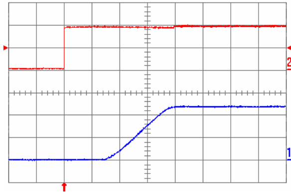
Fig. 1.2V.5: Turn-on transient for V_{out} = 1.2 V with the application of Enable signal at full rated load current (resistive) and 47 \mu F external capacitance at V_{in} = 5 V. Top trace: Enable signal (2 V/div.); Bottom trace: output voltage (500 mV/div.); Time scale: 2 ms/div.
