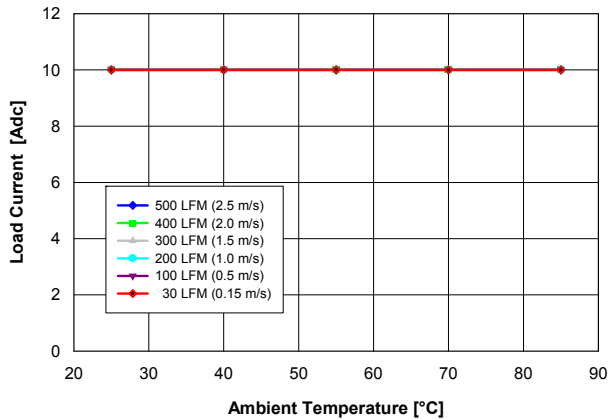
Fig. 2.5V.1: Available load current vs. ambient temperature and airflow rates for V_{out} = 2.5 V converter mounted vertically with V_{in} = 5 V, and maximum MOSFET temperature \leq 120 °C.
