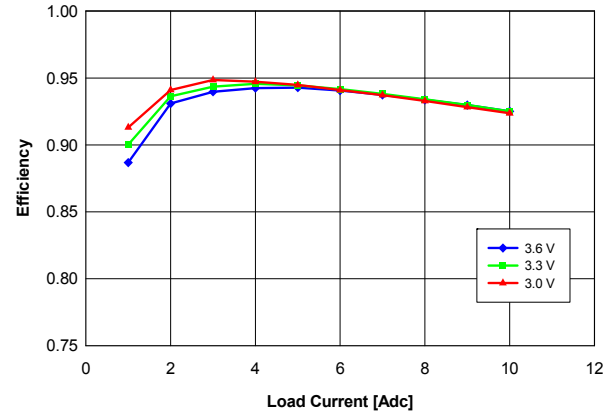
Fig. 2.0V.4: Efficiency vs. load current and input voltage for Vout = 2.0 V converter mounted vertically with air flowing at a rate of 200 LFM (1 m/s) and Ta = 25 °C.
