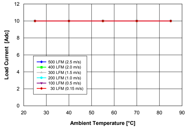
Fig. 3.3V.2: Available load current vs. ambient temperature and airflow rates for Vout = 3.3 V converter mounted horizontally with Vin = 5 V, and maximum MOSFET temperature ≤ 120 °C.
