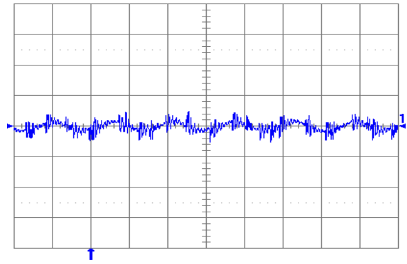
Fig. 1.8V.6: Output voltage ripple (20 mV/div.) at full rated load current into a resistive load with external capacitance 47\text{ }\mu\text{F} ceramic + 1\text{ }\mu\text{F} ceramic, and V_{in} = 5\text{ V} for V_{out} = 1.8\text{ V} . Time scale: 2 \mu\text{s} /div.
