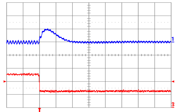
Fig. 1.0V.8: Output voltage response for V_{out} = 1.0 V to negative load current step change from 10 A to 5 A with slew rate of -5 \text{ A}/\mu\text{s} at V_{in} = 5 V. Top trace: output voltage (100 mV/div.); Bottom trace: load current (5 A/div.). C_o = 47 \mu\text{F} ceramic + 1 \mu\text{F} ceramic. Time scale: 20 \mu\text{s} /div.
