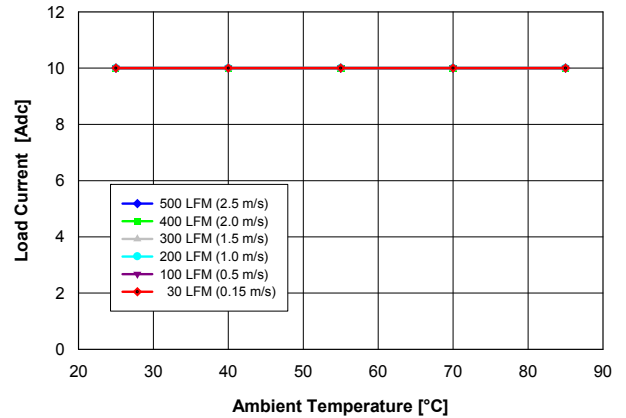
Fig. 2.0V.2: Available load current vs. ambient temperature and airflow rates for Vout = 2.0 V converter mounted horizontally with Vin = 5 V, and maximum MOSFET temperature ≤ 120 °C.
