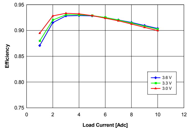
Fig. 1.5V.4: Efficiency vs. load current and input voltage for V_{out} = 1.5 V converter mounted horizontally with air flowing at a rate of 200 LFM (1 m/s) and T_a = 25 °C.
