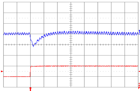
Fig. 3.3V.7: Output voltage for V_{out} = 3.3 V to positive load current step change from 5 A to 10 A with slew rate of 5 \text{ A}/\mu\text{s} at V_{in} = 5 V. Top trace: output voltage (100 mV/div.); Bottom trace: load current (5 A/div.). C_o = 47 \mu\text{F} ceramic + 1 \mu\text{F} ceramic. Time scale: 20 \mu\text{s} /div.
