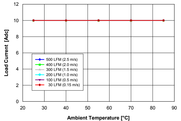
Fig. 1.8V.2: Available load current vs. ambient temperature and airflow rates for V_{out} = 1.8 V converter mounted horizontally with V_{in} = 5 V, and maximum MOSFET temperature \leq 120 °C.
