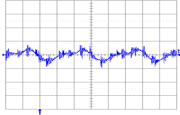
Fig. 2.5V.6: Output voltage ripple (20 mV/div.) at full rated load current into a resistive load with external capacitance 47 \mu F ceramic + 1 \mu F ceramic, and V_{in} = 5 V for V_{out} = 2.5 V. Time scale: 2 \mu s/div.
