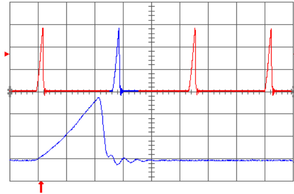
Fig. D: Output short circuit current (10 A/div) ( R_{LOAD} = 10\text{ m}\Omega ) for V_{out} = 5.0\text{ V} Time scale: 1 ms/div.; Bottom trace: Zoomed current with time scale 0.1 ms/div.
