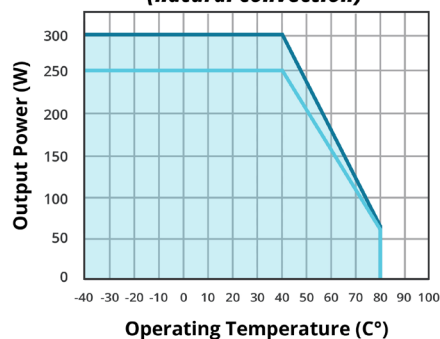
TEMPERATURE DERATING CURVE VMS-300A-CNF (natural convection)
