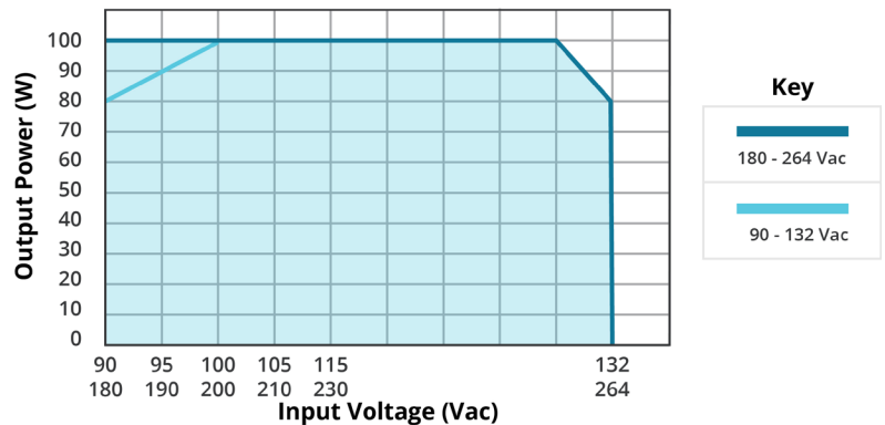
INPUT VOLTAGE DERATING CURVE (at 25°C)
