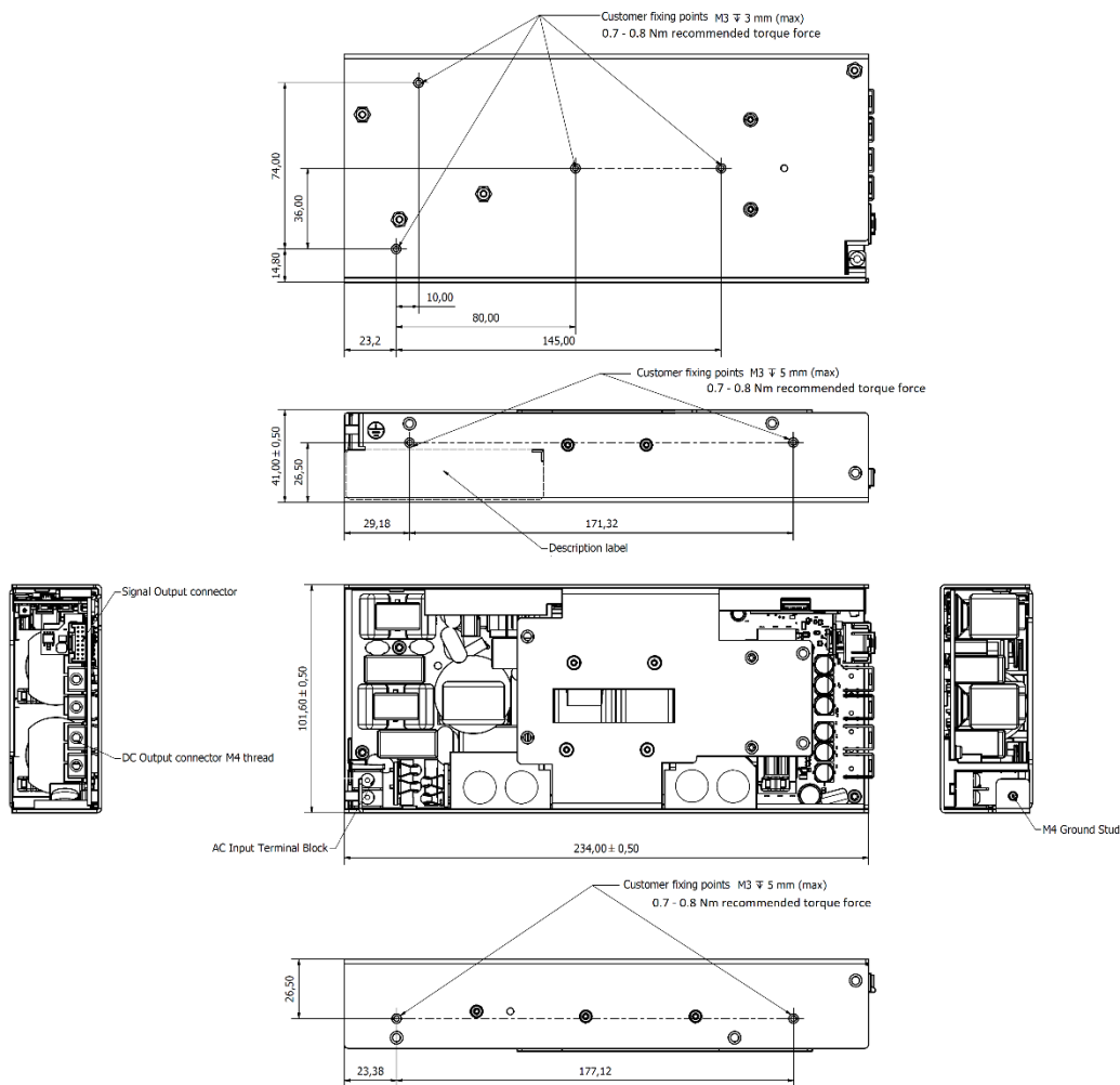
Figure 2. Mechanical Drawing – MCC750-1T24 / MCC750-1T48 Models
