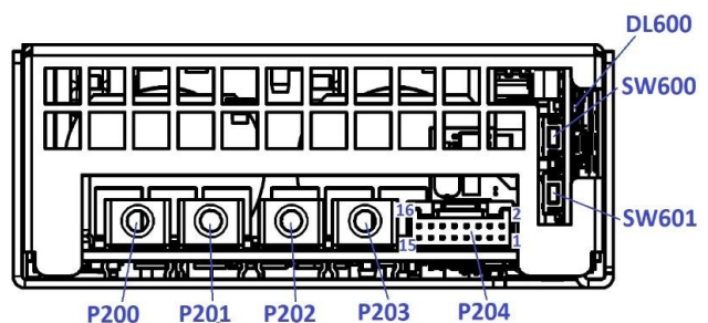
Figure 7. Rear View - MCC750-1T24-PC / MCC750-1T48-PC Models
