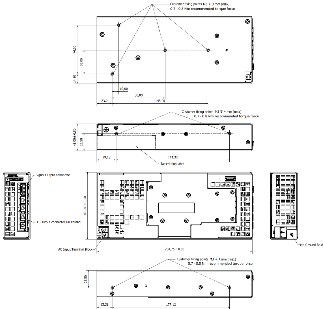
Figure 5. Mechanical Drawing - MCC750-1T24-PC / MCC750-1T48-PC Models
