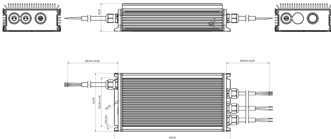
Figure 3. Mechanical drawing
