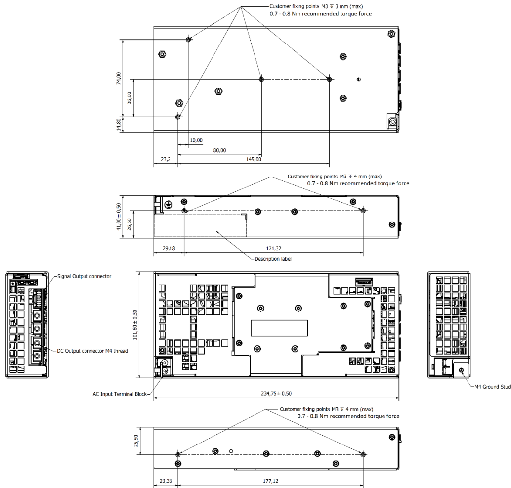
Figure 5. Mechanical Drawing - ACC750-1T24-PC / ACC750-1T48-PC Models
