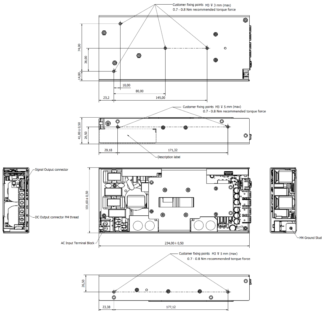
Figure 2. Mechanical Drawing – ACC750-1T24 / ACC750-1T48 Models
