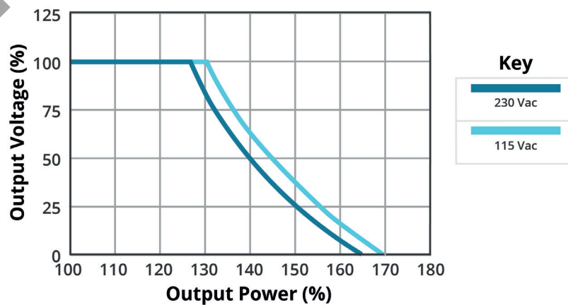
TYPICAL OVER CURRENT PROTECTION CURVE (PDRC-36-24)
