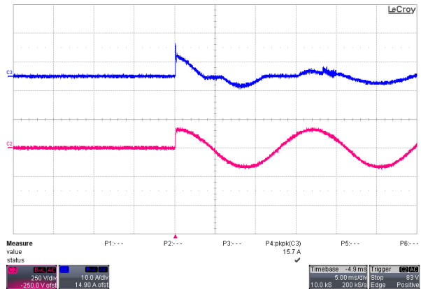
Figure 2: Inrush current, V_{in} = 115\text{Vac} , 90^\circ CH2: V_{in} (250V/div), CH3: I_{in} (10A/div)
