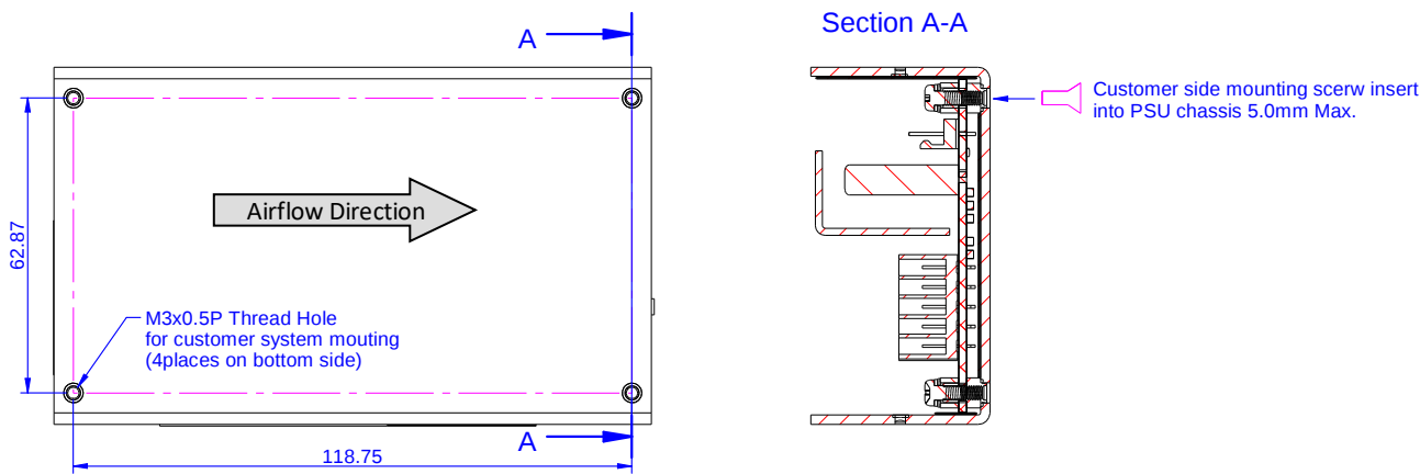
Figure 20: Bottom view 2
