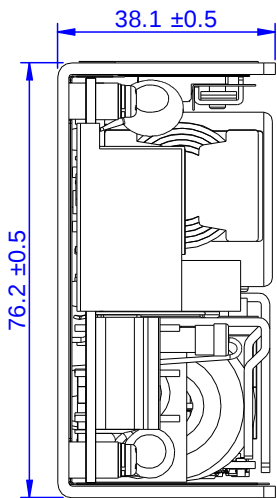
Figure 21: Front view
