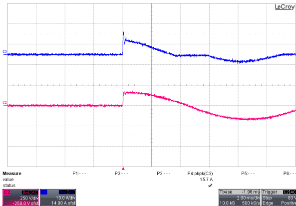
Figure 2: Inrush current, V_{in} = 115\text{Vac} , 90^\circ CH2: V_{in} (250V/div), CH3: I_{in} (10A/div)
