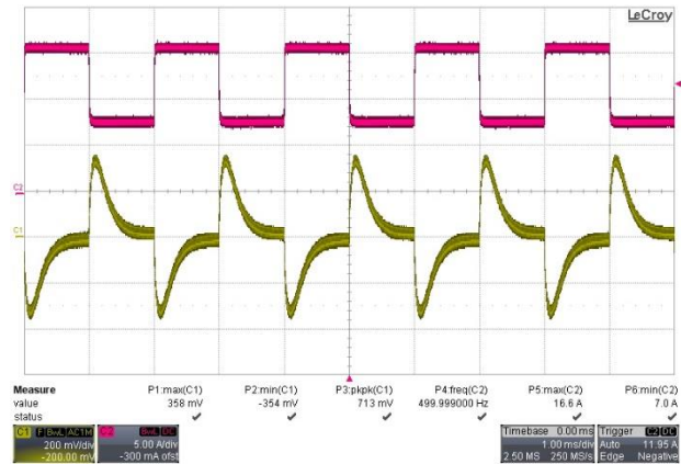
Figure 14: Load transient V_o (1.0ms/div), 8.5A <-> 17A, 2Aμs CH1: V_o (200 mV/div) CH2: I_o (5 A/div)
