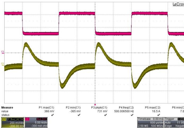
Figure 13: Load transient V_o (500μs/div), 8.5A <-> 17A 2Aμs CH1: V_o (200mV/div) CH2: I_o (5.0 A/div)
