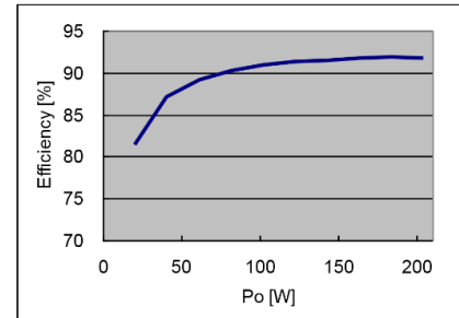
Efficiency vs. Output Power at 230VAC, ABC200-1048G
