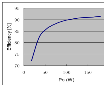
Efficiency vs. Output Power at 230VAC, ABC200-1012G
