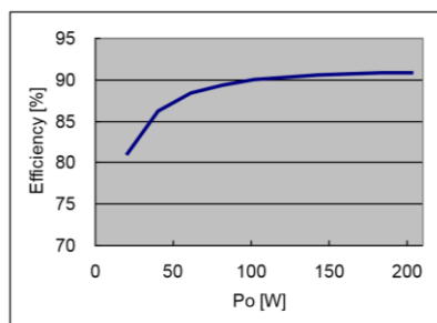
Efficiency vs. Output Power at 230VAC, ABC200-1024G
