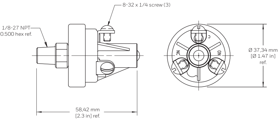
Figure 29. 5000 Series Dimensions
