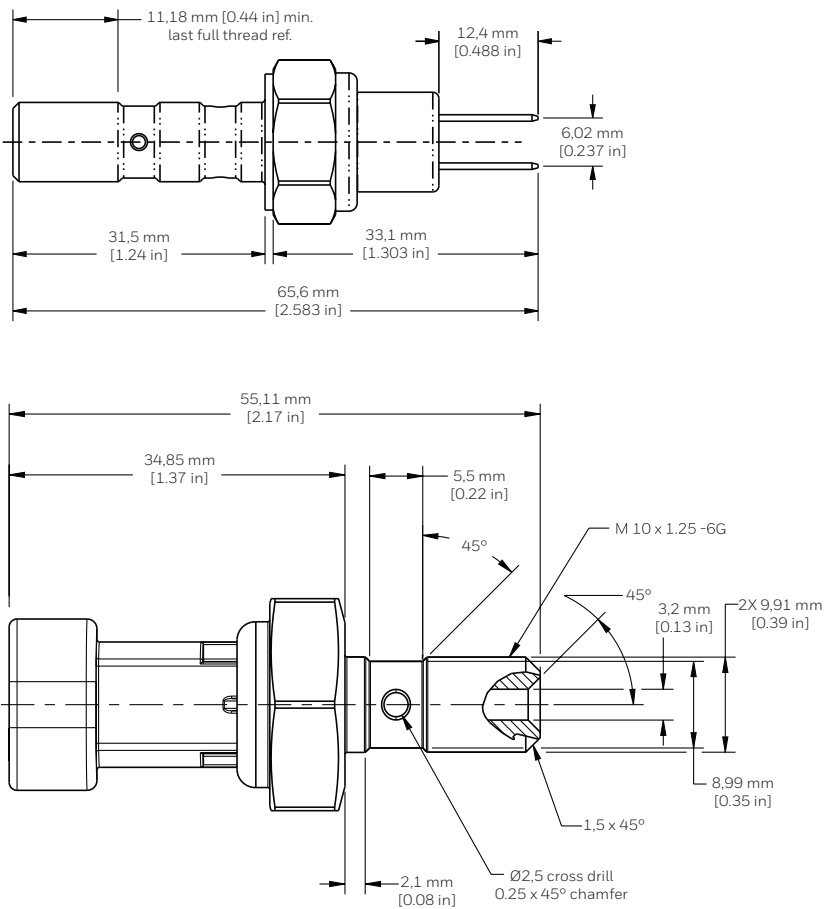
Figure 28. 1000 Series Dimensions
