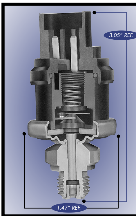
5000 Series Piston Switch with Metri-Pack Terminal
