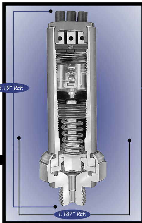
Diaphragm Type
