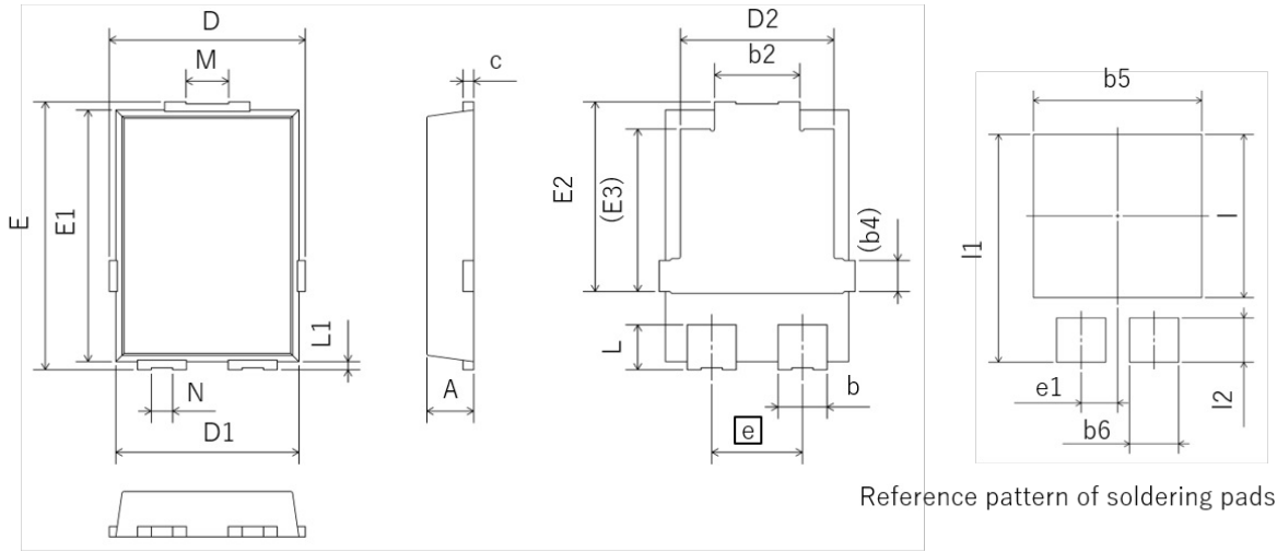
TO-277A, (TO-277GE)
