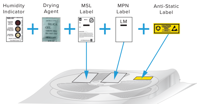
Vacuum bag.
