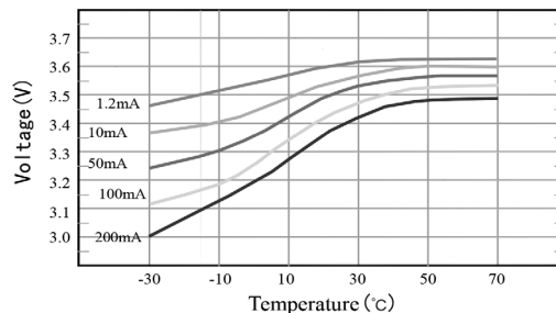
■ Voltage VS. Temperature
