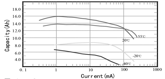
■ Capacity VS. Current
