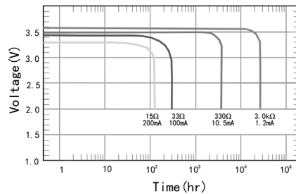
■ Discharge characteristics at 23±2°C
