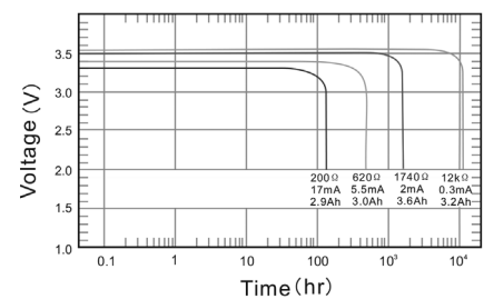
Discharge Characteristics at 23°C
