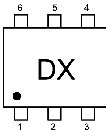
Fig. 6.1 Marking
