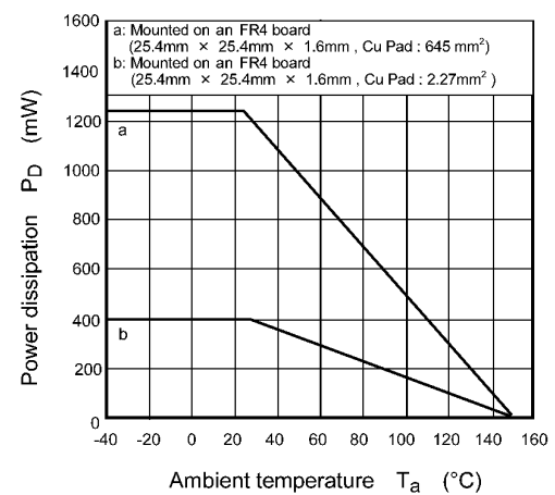
Fig. 8.12 P_D - T_a
