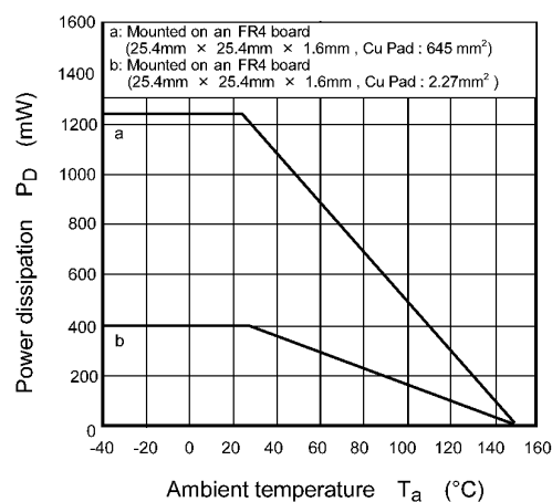
Fig. 8.6 P_D - T_a
