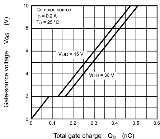
Fig. 7.9 Dynamic Input Characteristics
