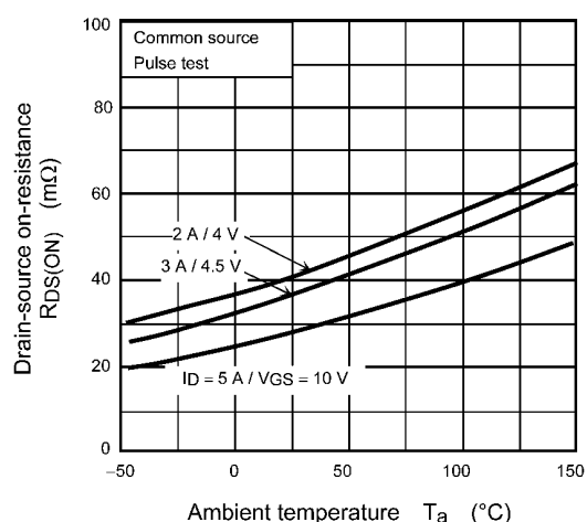
Fig. 8.5 R_{DS(ON)} - T_a
