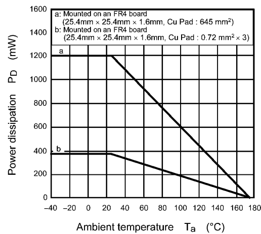
Fig. 8.13 P_D - T_a
