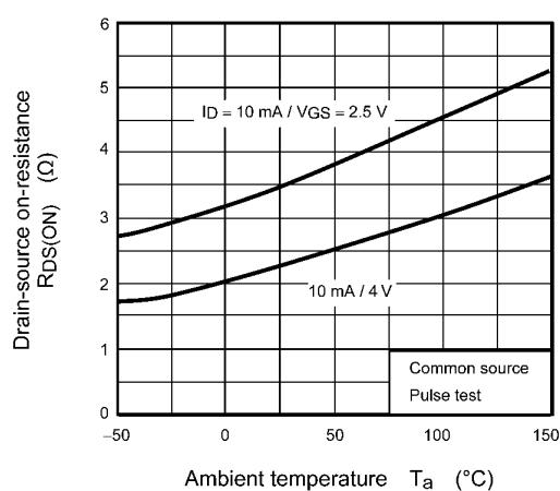
Fig. 8.5 R_{DS(ON)} - T_a
